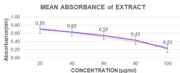
Fig. 4: Mean absorbance of O. gratissimum hydroalcoholic extract at different concentrations (20–100 \mu\text{g/mL} ) during the NO scavenging assay. A concentration-dependent decrease in absorbance was observed.
