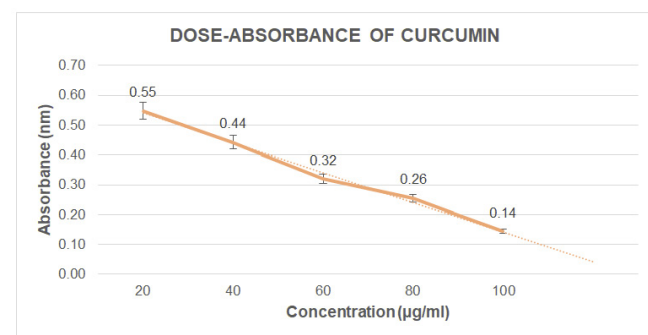
Fig. 6: Mean absorbance of curcumin at different concentrations (20 to 100 \mu\text{g/mL} ) during the NO scavenging assay. A concentration-dependent decrease in absorbance was observed, indicating increased nitric oxide scavenging assay with increasing extract concentration.
