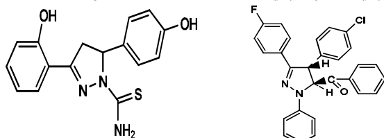
Fig.26. 3-(2-hydroxyphenyl)-5-(4-hydroxyphenyl)-2-pyrazolin-1-carbothioamide
