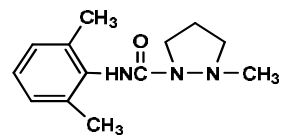
Fig.8b. N-(2,6-dimethylphenyl)-2-methylpyrazolidine-1-carboxamide
