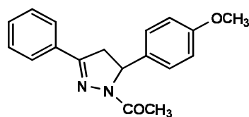
Fig.45. 1-(5-(4-methoxyphenyl)-3-phenyl-2-pyrazolin-1-yl)ethanone
