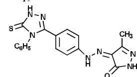
Fig.6. (Z)-3-methyl-4-(2-(4-(4-phenyl-5-thioxo-4,5-dihydro-1H-1,2,4-triazol-3-yl)phenyl)hydrazono)-1H-pyrazol-5(4H)-one
