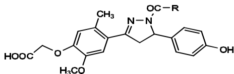
Fig.37. 2-(4-(5-(4-hydroxyphenyl)-1-(2-phenoxyacetyl)-2-pyrazolin-3-yl)-2-methoxy-5-methylphenoxy)acetic acid, where, R=CH 2 OC 6 H 5 ; 2-(4-(1-alkylacetoxy-5-(4-hydroxyphenyl)-2-pyrazolin-3-yl)-2-methoxy-5-methylphenoxy)acetic acid, where, R=CH 2 OC 10 H 7
