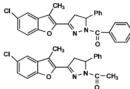
Fig.31. 3-(5-chloro-3-methylbenzofuran-2-yl)-5-phenyl-2-pyrazolin-1-yl(phenyl)methanone; 1-(3-(5-chloro-3-methylbenzofuran-2-yl)-5-phenyl-2-pyrazolin-1-yl)ethanone
