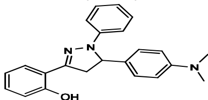
Fig.12. 2-(5-(4-(dimethylamino)phenyl)-3-phenyl-2-pyrazolin-3-yl)phenol
