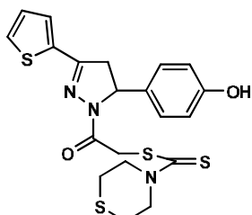
Fig.36. 2-(5-(4-hydroxyphenyl)-3-(thiophen-2-yl)-2-pyrazolin-1-yl)-2-oxoethyl thiomorpholine-4-carbodithioate
