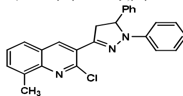
Fig.30. 2-chloro-3-(1,5-diphenyl-2-pyrazolin-3-yl)-8-methylquinoline
