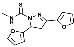
Fig.4. 3,5-di(furan-2-yl)-N-methyl-2-pyrazolin-1-carbothioamide
