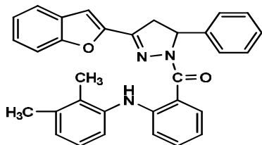
Fig.44b. 3-(benzofuran-2-yl)-5-phenyl-2-pyrazolin-1-yl(2-(2,3-dimethylphenylamino)phenyl)methanone
