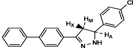
Fig.17. 3-(biphenyl-4-yl)-5-(4-chlorophenyl)-2-pyrazoline
