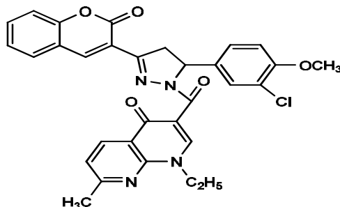
Fig.48. 3-(5-(3-chloro-4-methoxyphenyl)-3-(2-oxo-2H-chromen-3-yl)-2-pyrazolin-1-carbonyl)-1-ethyl-7-methyl-1,8-naphthyridin-4(1H)-one
