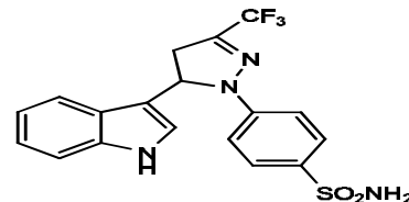
Fig.62. 4-(5-(1 H -indol-3-yl)-3-(trifluoromethyl)-2-pyrazolin-1-yl)benzenesulfonamide
