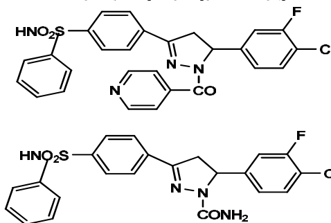
Fig.33. 5-(4-chloro-3-fluorophenyl)-3- p -benzenesulphonamido-2-pyrazolin-1-yl(pyridin-4-yl)methanone; 5-(4-chloro-3-fluorophenyl)-3- p -benzenesulphonamido-2-pyrazolin-1-carboxamide
