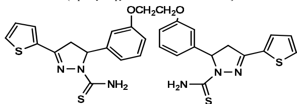
Fig.16b. 5,5'-(3,3'-(ethane-1,2-diylbis(oxy))bis(3,1-phenylene)) bis(3-(thiophen-2-yl)-2-pyrazolin-1-carbothioamide)
