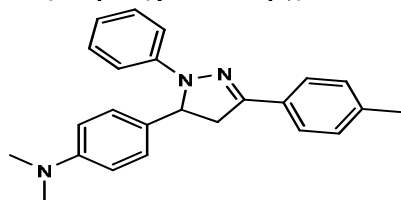
Fig.13. N,N -dimethyl-4-(1-phenyl-3- p -tolyl-2-pyrazolin-5-yl)aniline
