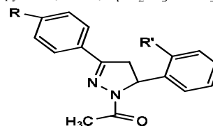
Fig.41. 1-(3,5-diphenyl-2-pyrazolin-1-yl)ethanone, where, R=R'=H; 1-(5-(2-methoxyphenyl)-3-phenyl-2-pyrazolin-1-yl)ethanone, where, R=H, R'=OCH 3
