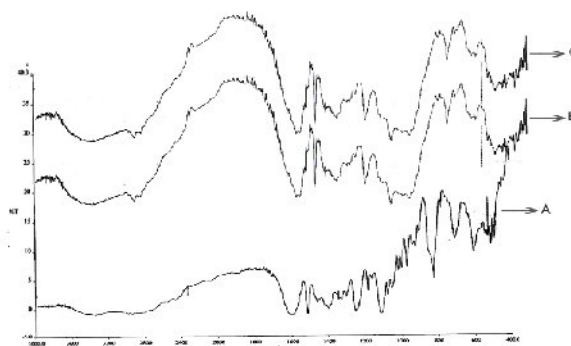
Fig.1: FT-IR spectra of pure Metoprolol tartrate (A), powdered sample of matrix tablets M3 (B) and triple-layer matrix tablets M3L3 (C)
