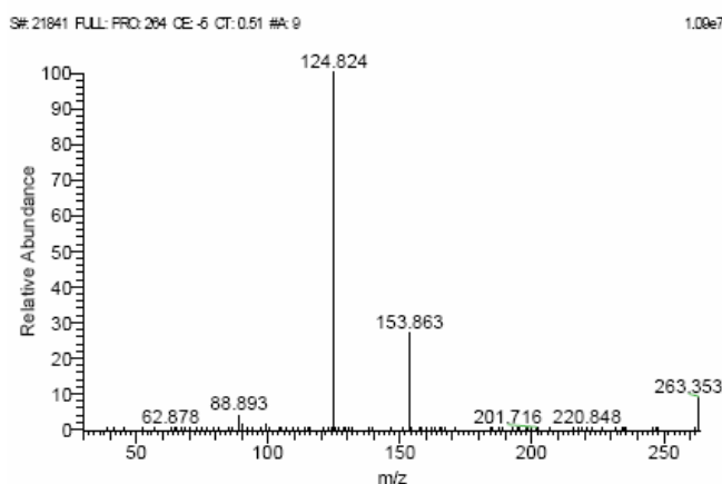
(b) Ticlopidine full scan mass spectra
