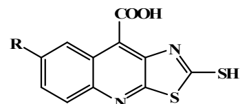
6b R=H, Br, NO 2
