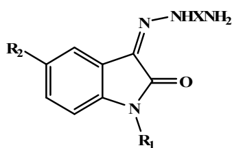
2(a-c) R 1 =H, CH 3 , H, R 2 =H, X=O, O, S
