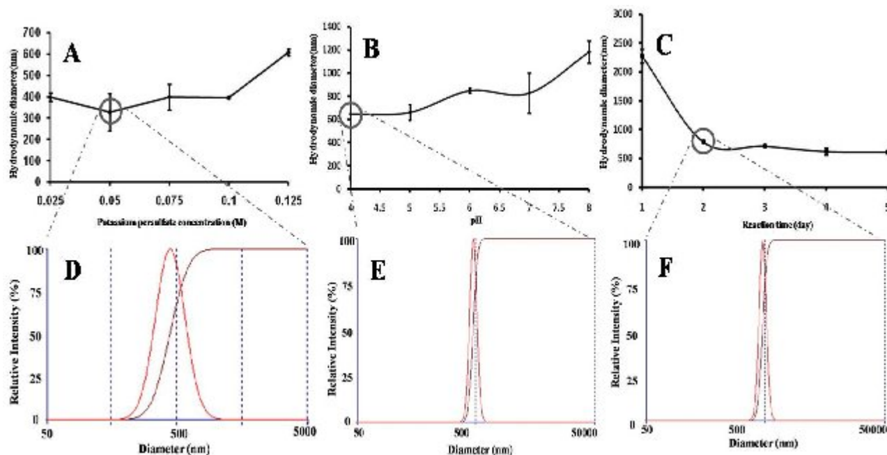
Fig. 1: Effect of K_2S_2O_8 concentration, pH and reaction time on in vitro depolymerisation of native chitosan. (A) HD profile on K_2S_2O_8 concentration, (B) HD profile on pH, (C) HD profile on reaction time, (D) HD distribution of depolymerised chitosan at optimized 0.05 M potassium persulfate concentration, (E) HD distribution of depolymerised chitosan at optimized pH 4, (F) HD distribution of depolymerised chitosan at optimized reaction time 2 days
