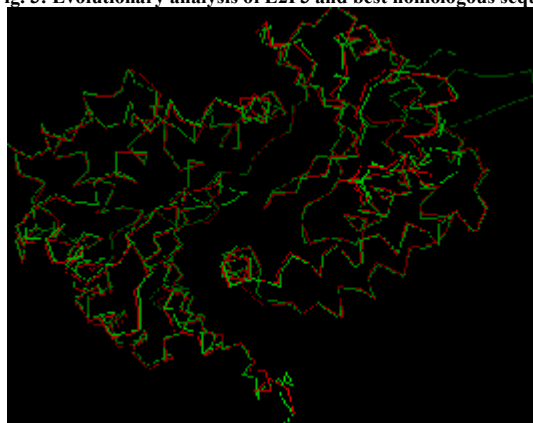
Fig. 4: Superimposed structure of E2F3 and template
