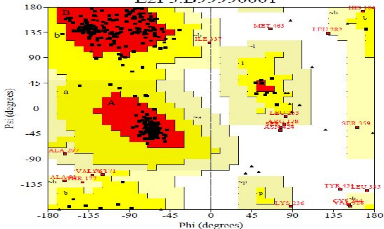
Fig. 8: Ramachandran plot generated by PROCHECK
