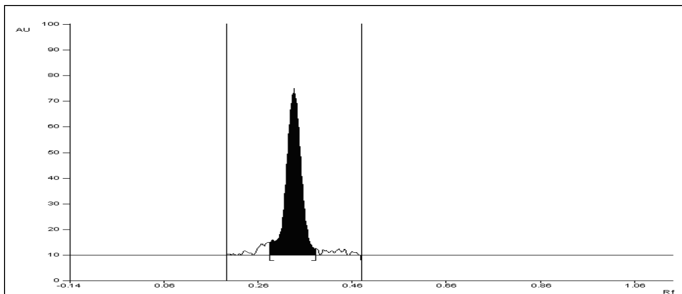
Fig. 1: Representative Chromatogram of Isolated Standard Wedelolactone
