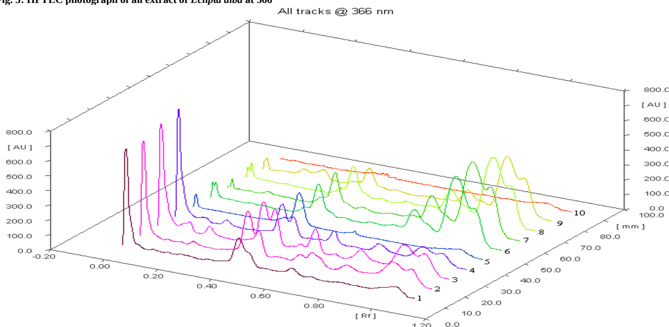
1: Maceration; 2: Soxhlet apparatus; 3: orbital shaker; 4: ultra sonication; 5: Standard wedelolactone; 6-10 (supercritical fluid extraction) Fig. 6: HPTLC 3D picture of all extract of Eclipta alba at 366nm
