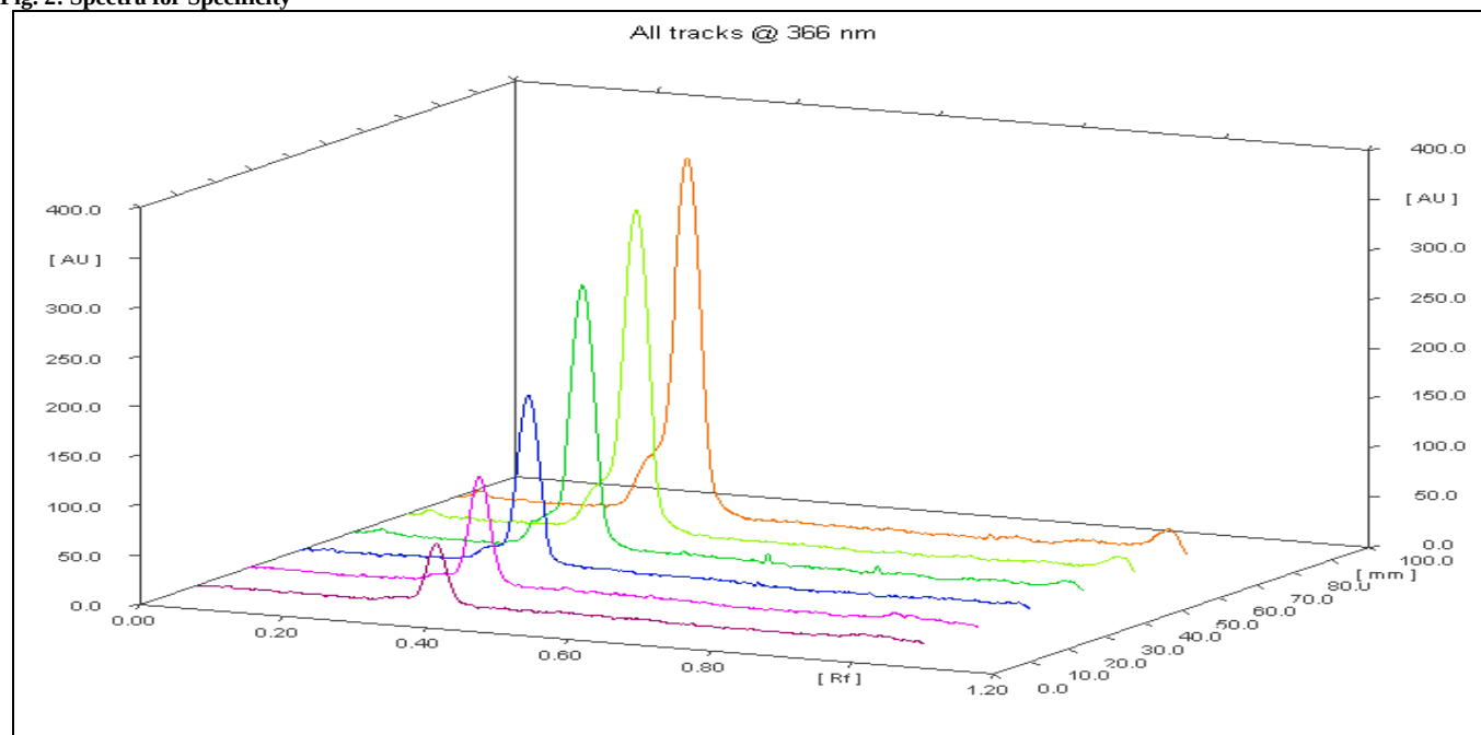
Fig. 3: Chromatogram of Standard at Different Concentration
