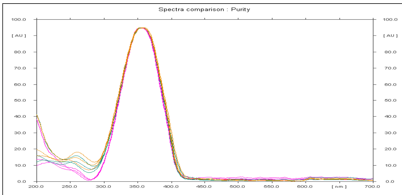
Fig. 4: Spectra for Peak Purity
