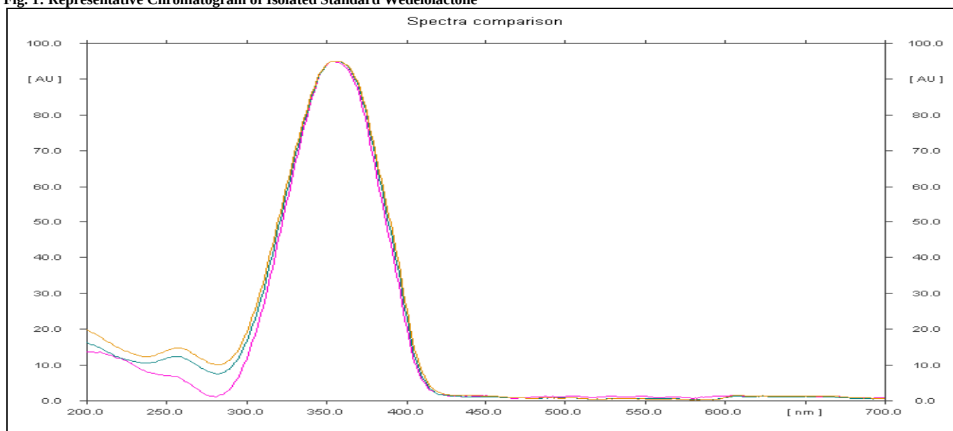
Fig. 2: Spectra for Specificity
