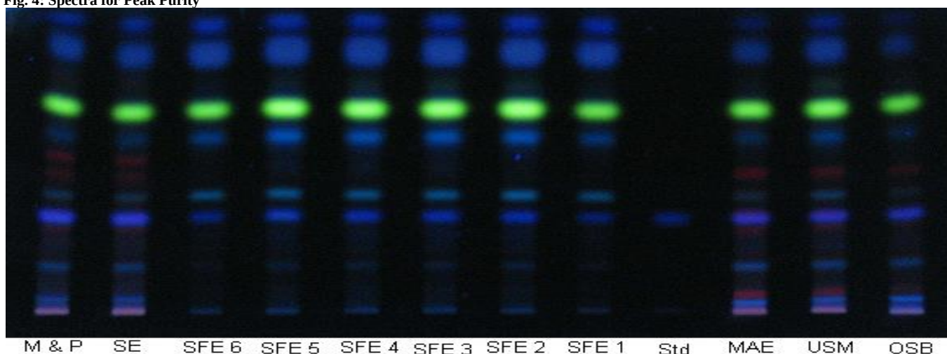
Fig. 5: HPTLC photograph of all extract of Eclipta alba at 366
