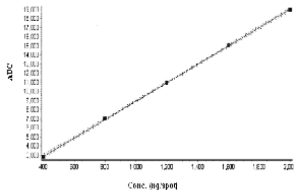
Fig. 3: Calibration Curve for HCTZ
