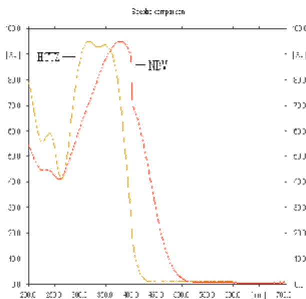
Fig. 4: Typical overlain spectra of standard NBV and HCTZ drug solutions
