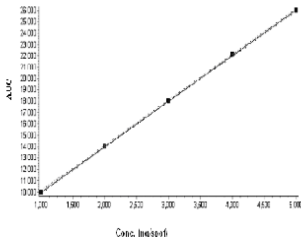
Fig. 2: Calibration curve for NBV
