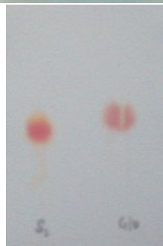
S 1 - L-glutamine Catalyzed by L-glutaminase for the formation of glutamic acid and S 2 - Standard glutamic acid
