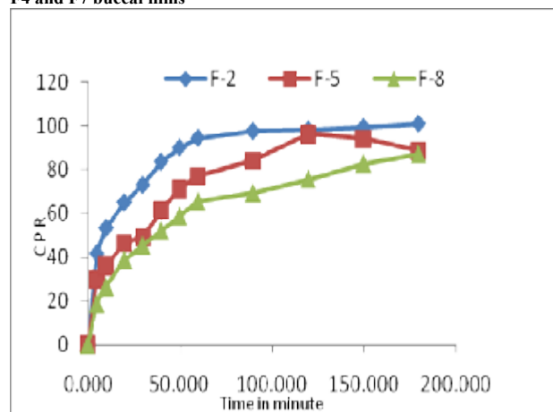
Fig. 6: Graph showing Cumulative percentage Release of Rasagiline Mesylate from Buccal films F2, F5 and F8
