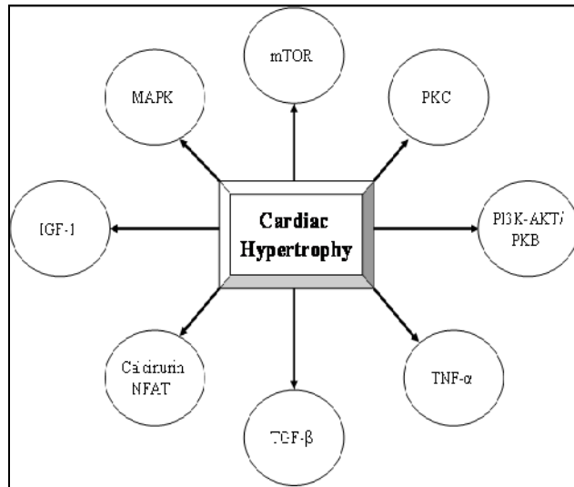
Fig. 1: Diagram showing signaling pathways of Cardiac Hypertrophy MAPK-mitogen-activated protein kinase; PKC-Protein kinase C; IGF-1-Insulin-like growth factor-I; (PI3K)-AKT/PKB phosphatidylinositol 3-kinase-Akt/Protein Kinase B; Calcineurin NFAT-nuclear factor of activated T cells; mTOR-mammalian target of rapamycin; TNF- \alpha -tumor necrotic factor-alpha; TGF- \beta -Transforming growth factor-beta
