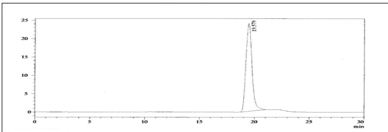
Fig. 2(a): HPLC Chromatogram of Reference Standard (Scopoletin)
