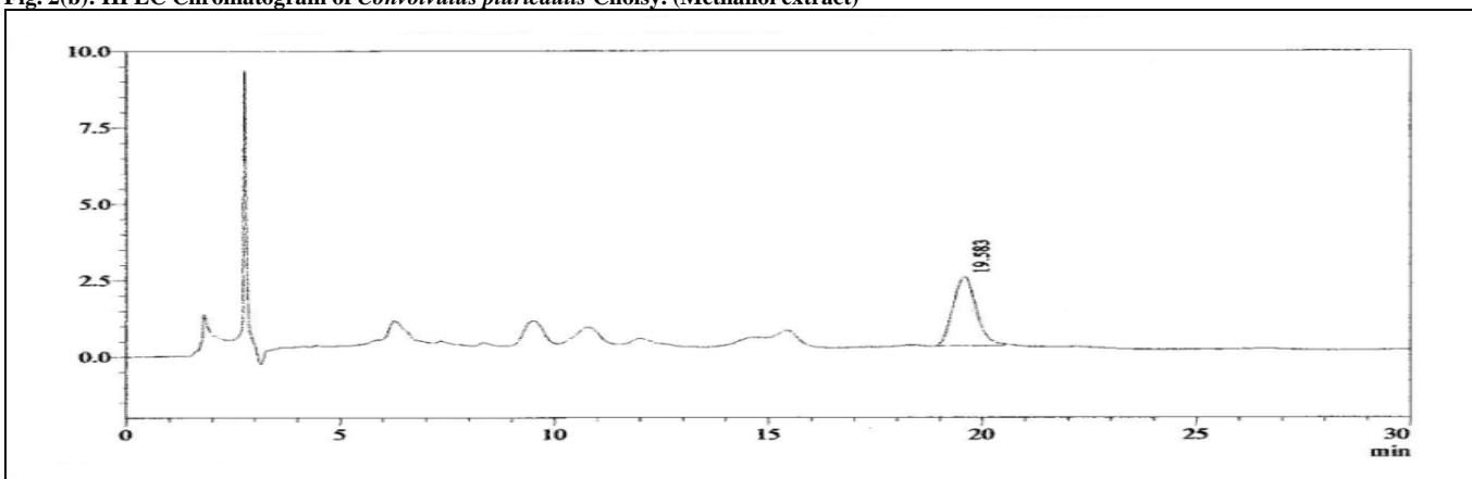
Fig. 2(c): HPLC Chromatogram of Convolvulus pluricaulis Choisy. (Hydro-alcoholic extract)
