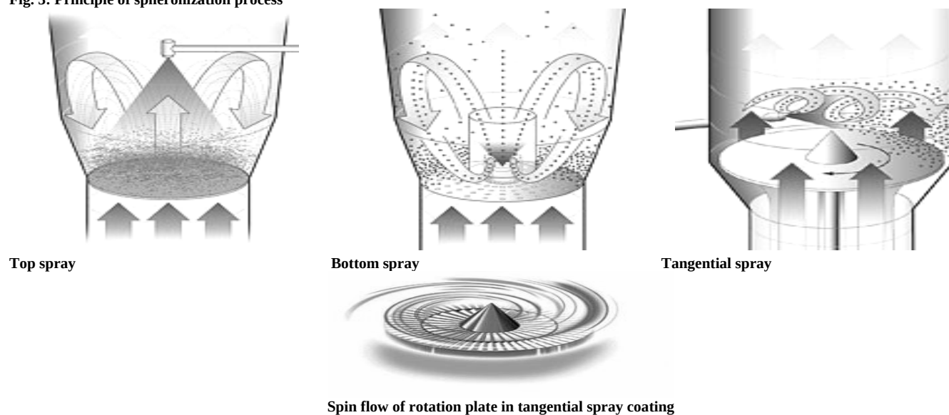
Fig. 3: Principle of spheronization process
