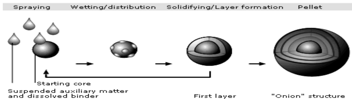
Fig. 1: Principle of solution and suspension layering
