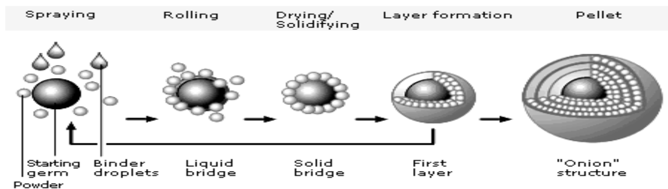
Fig. 2: Principle of powder layering
