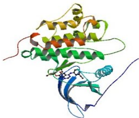
Fig. 1: The Crystal structure of the targets 1M17
