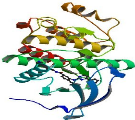
Fig. 2: The Crystal structure of the targets 3CS9
