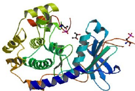
Fig. 3 The Crystal structure of the targets 3OVV
