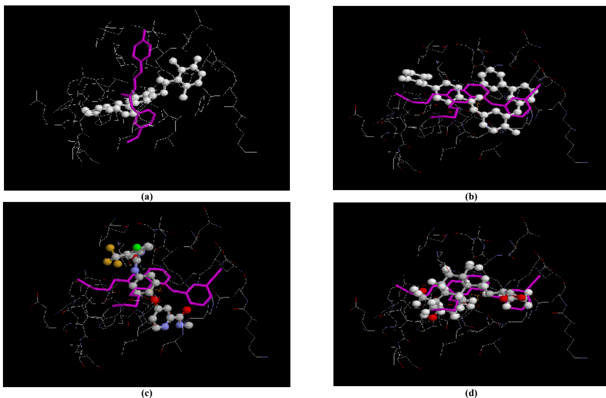
Fig. 7: Results of the docked structures with the target
