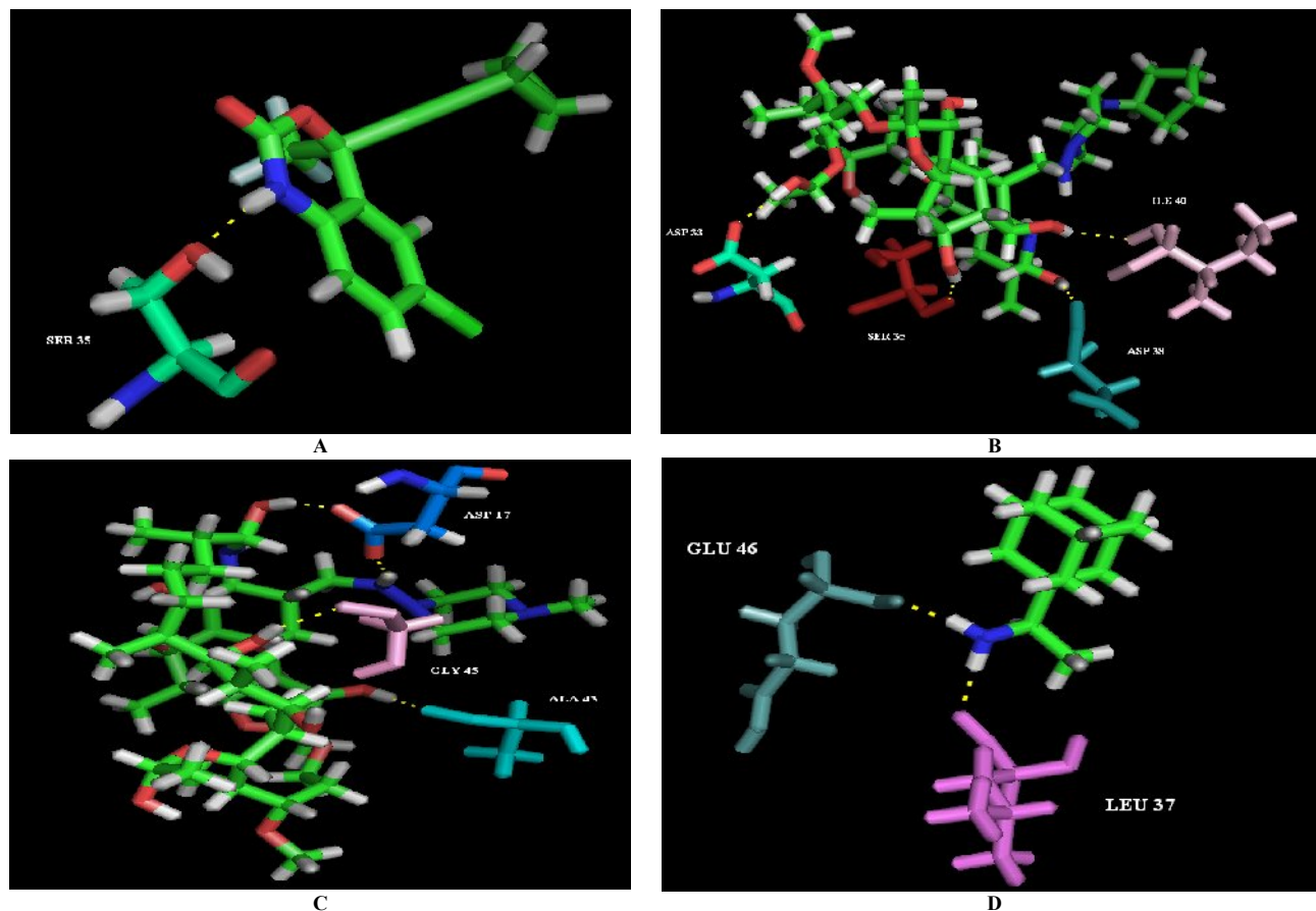
Fig. 2: Interaction between A) Efavirenz and RdRp B) Rifapentine and RdRp C) Rifampin and RdRp, D) Rimantadine and RdRp
