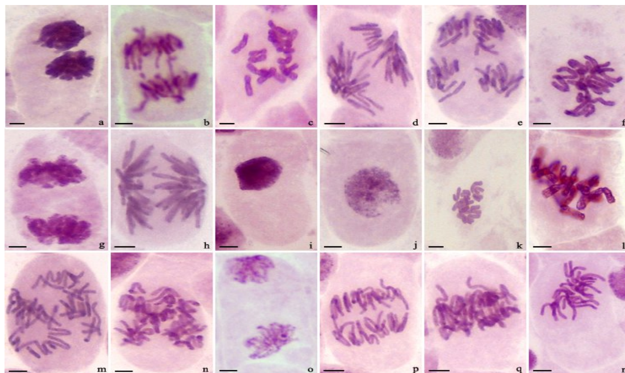
Fig. 1: Different Chromosomal aberrations induced by S. heyneanus root methanolic extract in root tip cells of A. cepa .
