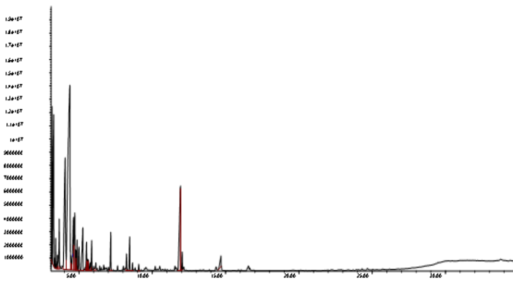
Fig. II: Gas chromatogram of tangerine oil extracts showing the various constituents
