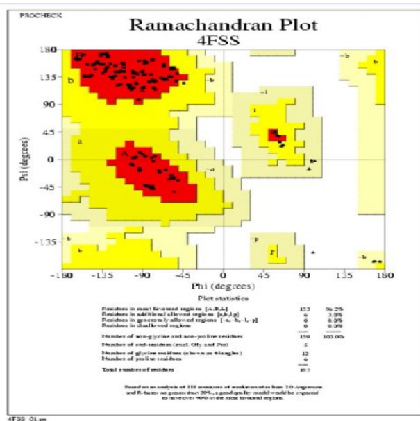
Fig. 1: Ramachandran Plot of 4FSS, 3096 and 4AQ3
