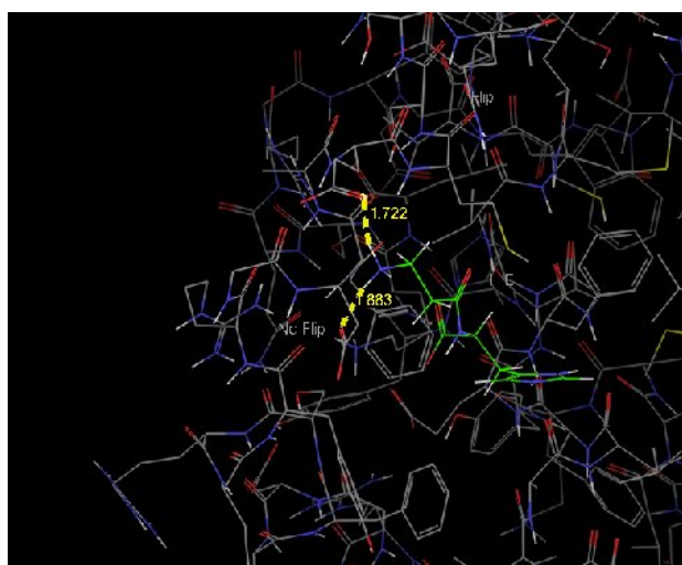
Fig. 3: Docking interaction of lead compounds with target proteins RAS P21 protein (4FSS), AKT-1 (3O96) and BLC-2 (4AQ3) proteins
