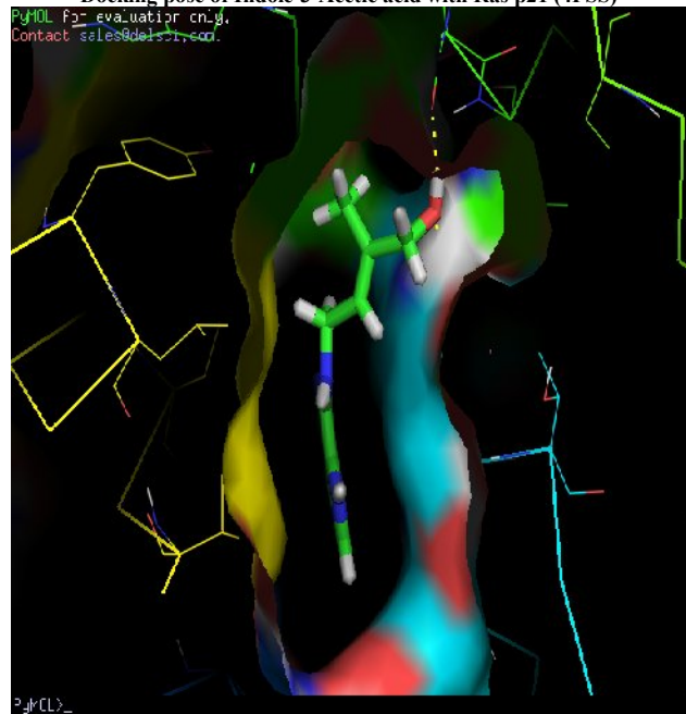
Docking pose of Zeatin with AKT-1 (3O96)
