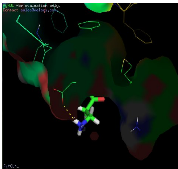
Docking pose of L-Histidine with 4AQ3
