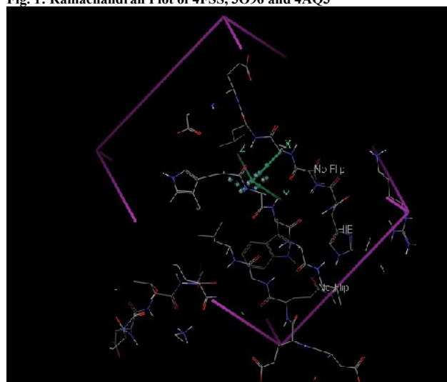
Site Map of RAS p21 Protein (4FSS.pdb)
