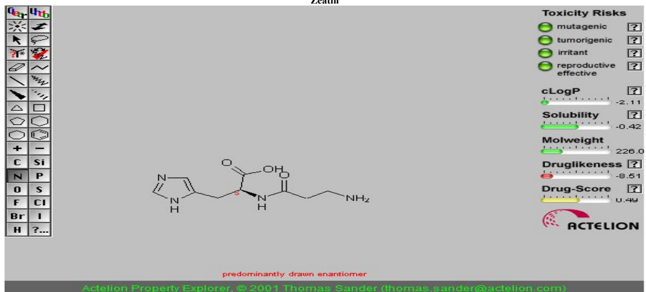
Fig. 5: Toxicity predicted for Indole-3-Acetic Acid, Zeatin and L-Histidine
