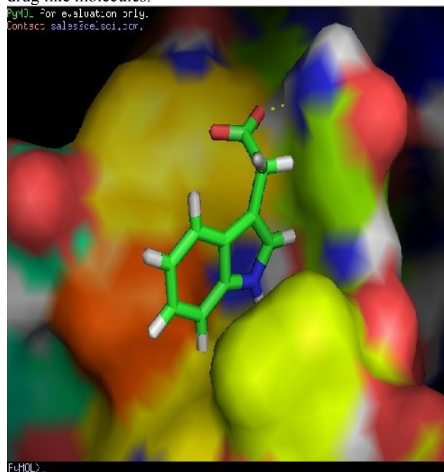
Docking pose of Indole-3-Acetic acid with Ras p21 (4FSS)
