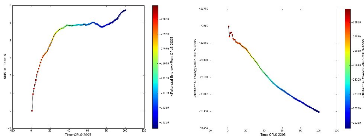
Fig. 6: RMSD of the backbone atoms of the docked 4AQ3 over a time period of 100 picoseconds
