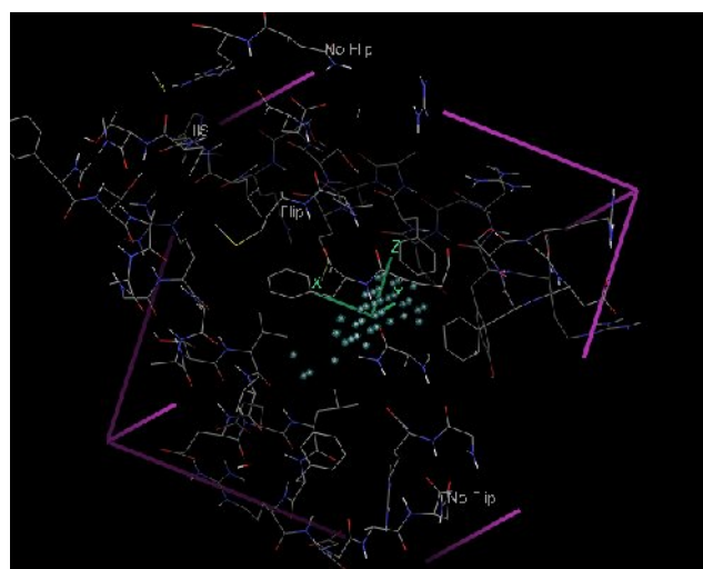
Site Map of BCL-2 (4AQ3.pdb)
