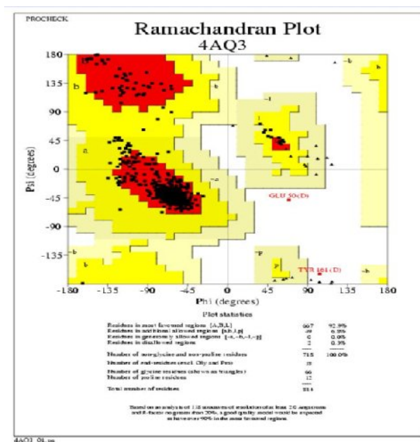
Fig. 1: Ramachandran Plot of 4FSS, 3096 and 4AQ3
