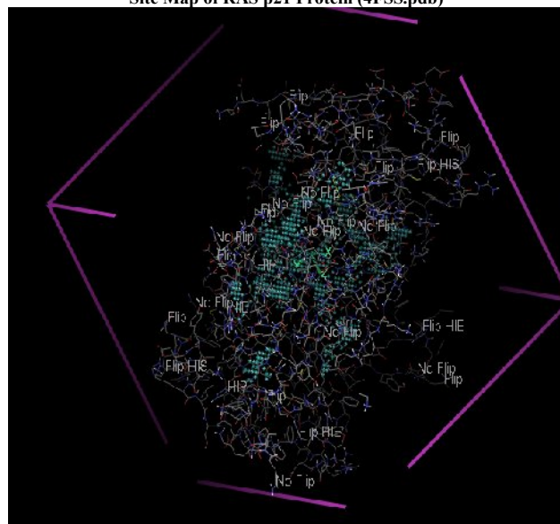
Site Map of AKT-1 (3096.pdb)
