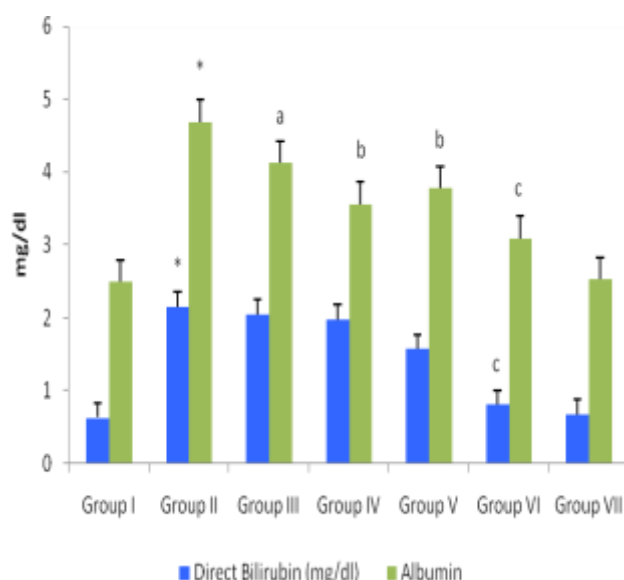
Fig. I: Effect Of MEWV On Albumin And Direct Bilirubin In \text{Al}_2(\text{SO}_4)_3 Induced Rats
