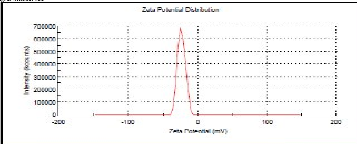
Fig. 3: Zeta potential
