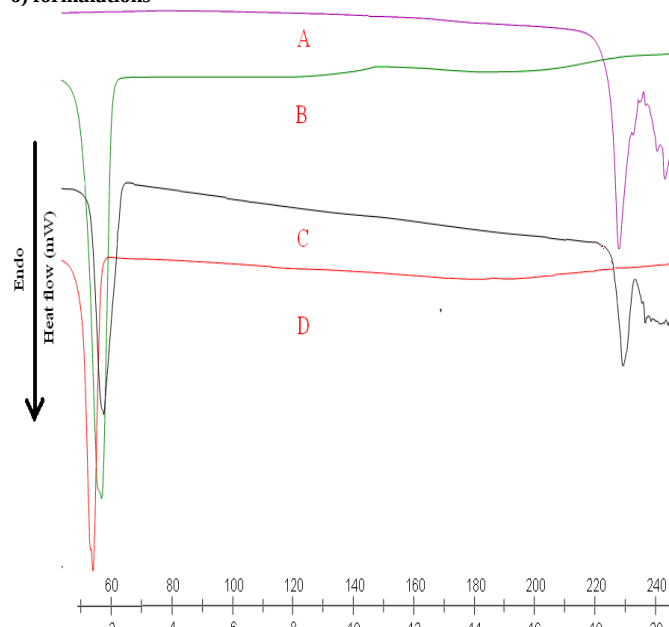
Fig. 5: DSC thermograms of LTZ (A), trimyrustin (B), physical mixture of LTZ and TM (C), and lyophilized LTZ-SLN (D)
