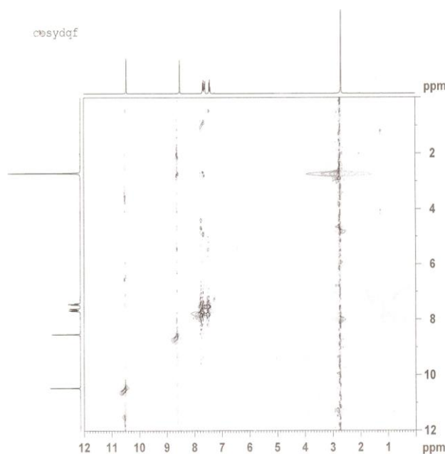
Fig. 4: COSY-DQF-Contour plot of 2-chloro-8-methyl-3-formylquinoline
