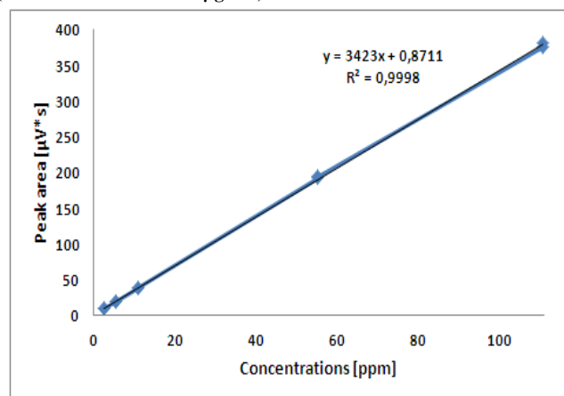
Fig. 2: Linearity curve of 2-propanol
