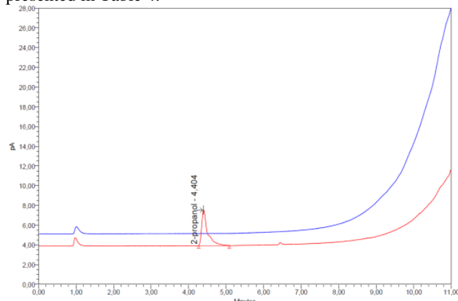
Fig. 1: Chromatograms of blank (water) and standard 2-propanol (concentration about 11.1 µg/mL)
