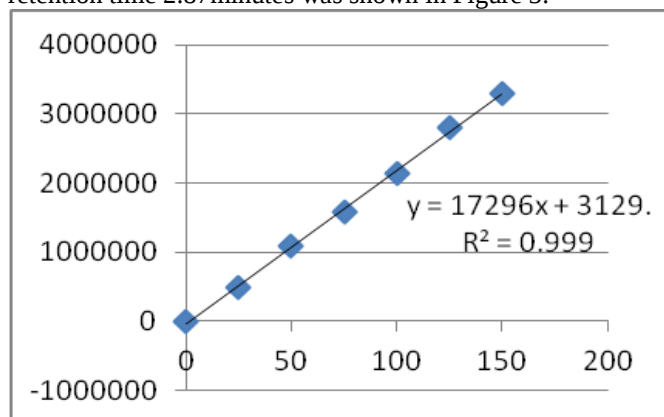
Fig. 2: Calibration curve of Dapagliflozin of Method A
