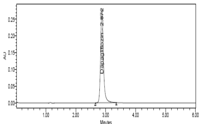
Fig. 3: Chromatogram of Dapagliflozin standard solution
