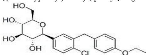
Fig. 1: Structure of Dapagliflozin
