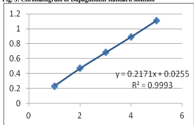
Fig. 4: Calibration curve of Dapagliflozin of UV spectroscopic method
