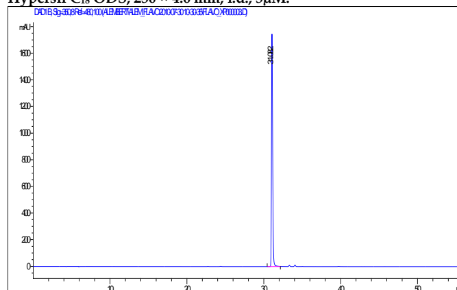
Fig. 6: HPLC chromatogram of compound 3 (350 nm); Column: Hypersil C 18 ODS, 250 × 4.6 mm, i.d., 5 µM.
