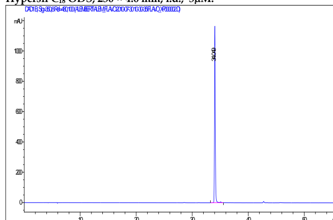
Fig. 5: HPLC chromatogram of compound 2 (350 nm); Column: Hypersil C 18 ODS, 250 × 4.6 mm, i.d., 5 µM.
