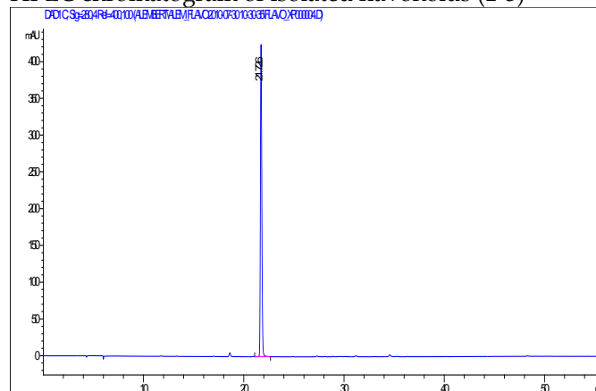
Fig. 4: HPLC chromatogram of compound 1 (280 nm); Column: Hypersil C 18 ODS, 250 × 4.6 mm, i.d., 5 µM.
