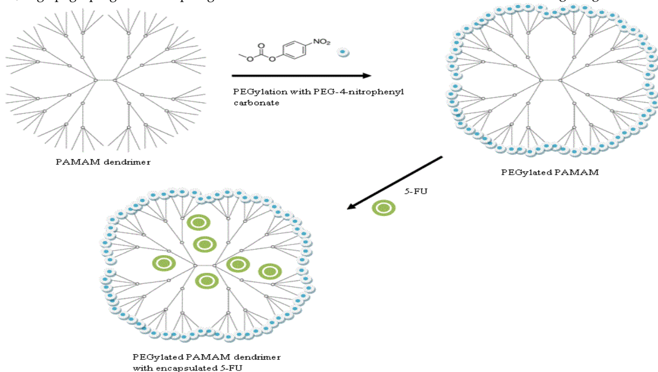
Fig. 2: PAMAM dendrimer PEGylation with PEG-4-nitrophenyl carbonate and encapsulation of 5-fluorouracil within PEG-PAMAM dendrimer
