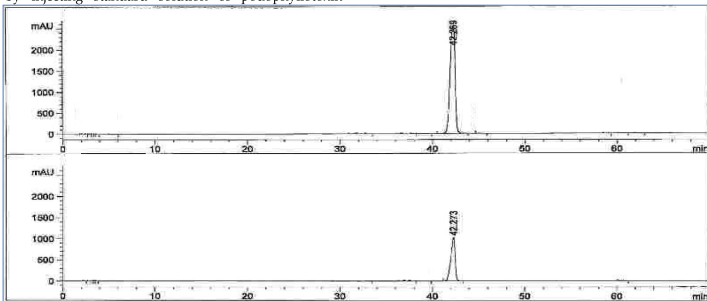
Fig. 1: HPLC chromatogram of standard podophyllotoxin.
