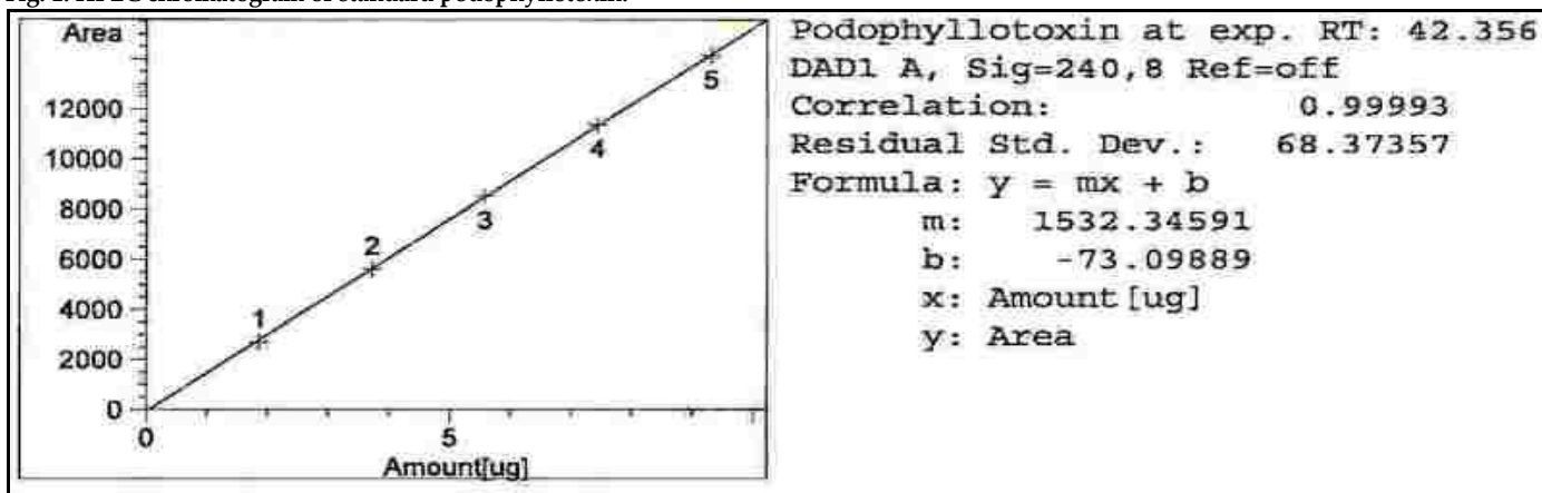
Fig. 2: Calibration curve for quantification of podophyllotoxin.
