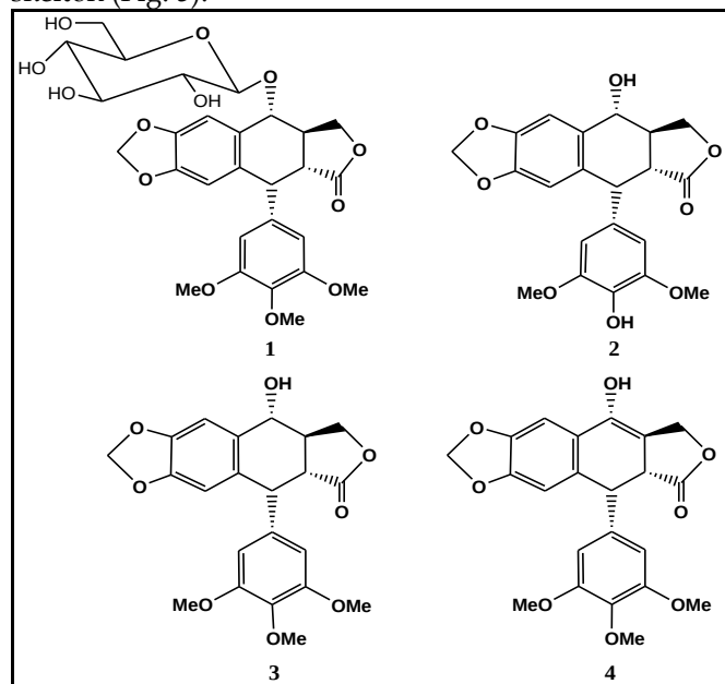
Fig. 5: Aryltetralin Lignans identified from rhizomes of Podophyllum hexandrum .
