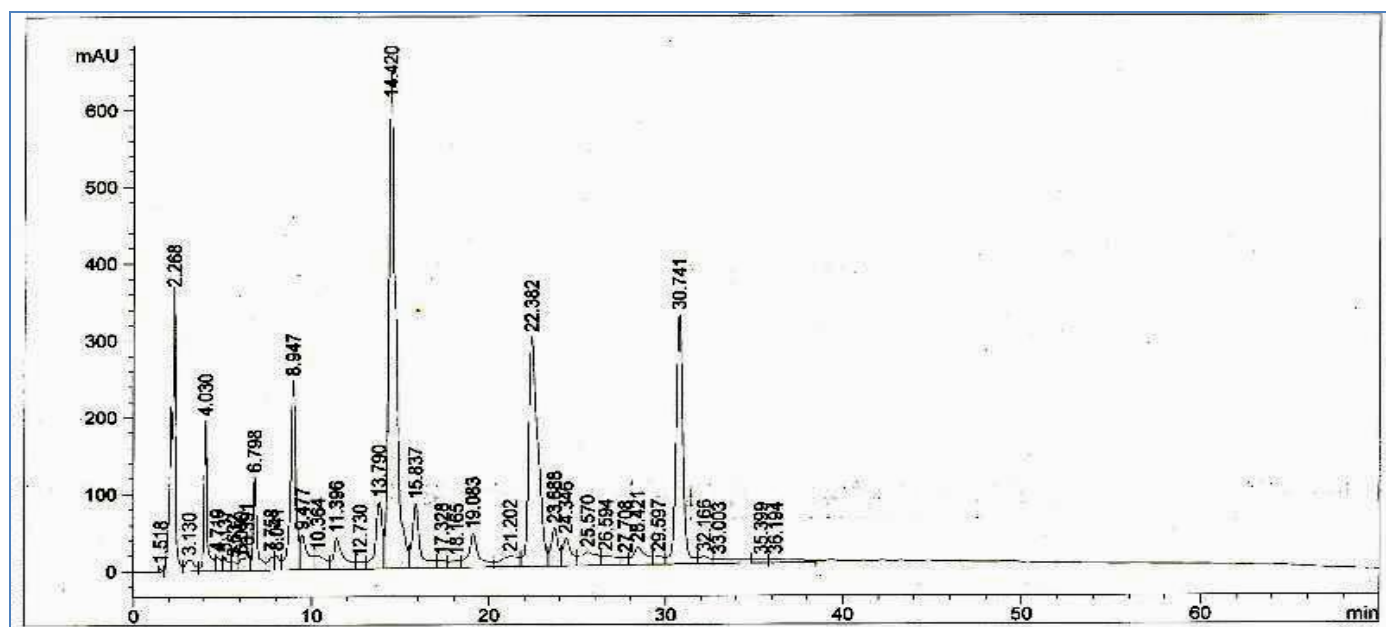
Fig. 3: HPLC chromatogram of methanolic extract from rhizomes of Podophyllum hexandrum .
