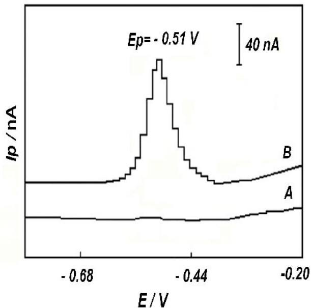
Fig. 2: Typical voltammogram of (A) 0.1 M Acetate buffer with pH 5.0 and (B) with 20 µg Nifedipine
