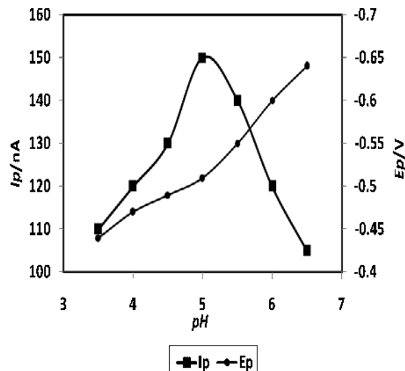
Fig. 1: Effect of pH on peak current ( I_p ) and peak potential ( E_p )
