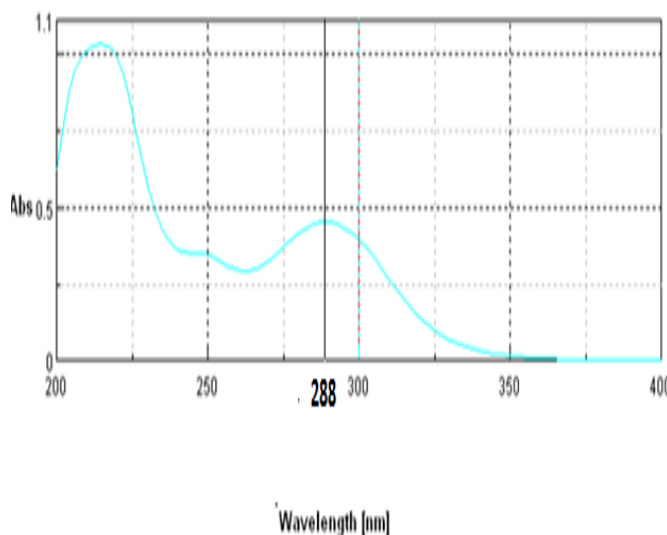
Fig. 2: UV spectrum of Dronedarone Hydrochloride (10 µg/ml)
