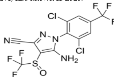
Fig. 1: Structure of Fipronil
