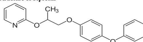
Fig. 2: Structure of Pyriproxyfen
