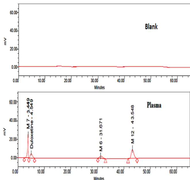
Fig. 5: Representative HPLC chromatograms of duloxetine and its metabolites present in rabbit plasma.
