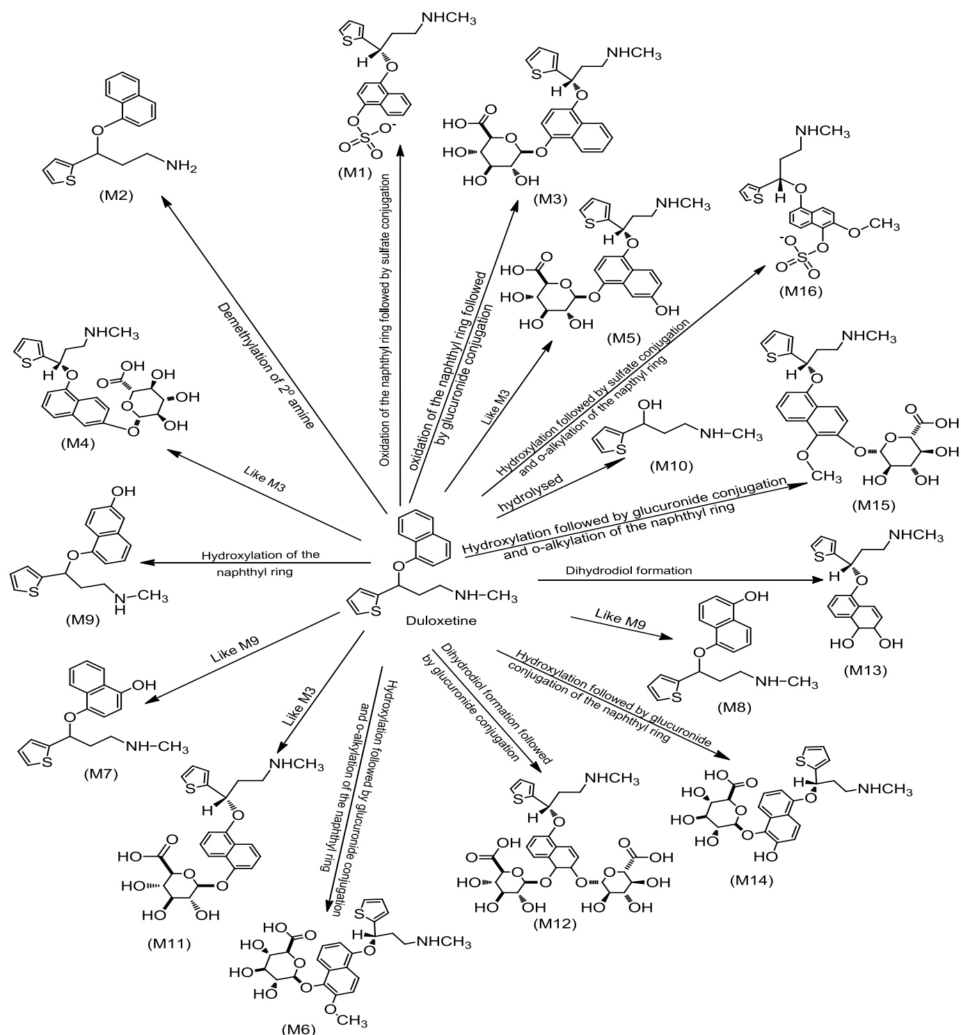
Fig. 1: Proposed in vivo metabolic scheme of duloxetine in rabbit after oral administration.
