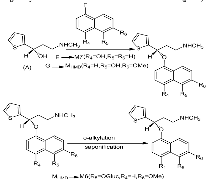
Fig. 3: Synthetic scheme for the metabolites of duloxetine (part-II).
