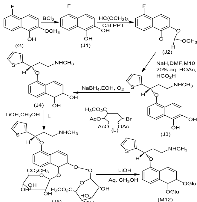
Fig. 4: Synthetic scheme for the metabolites of duloxetine (part-III).
