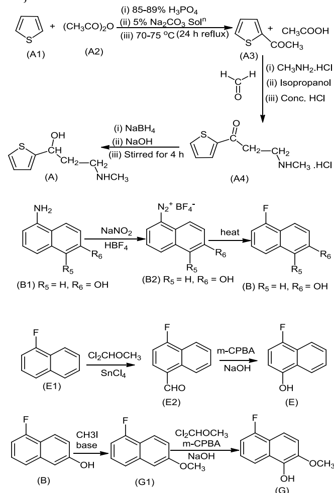
Fig. 2: Synthetic scheme for the metabolites of duloxetine (part-I).
