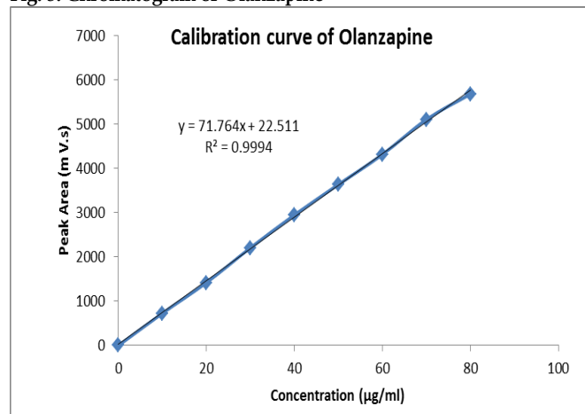
Fig. 4: Calibration curve of Olanzapine
