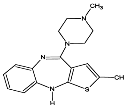
Fig. 1: Structure of Olanzapine
