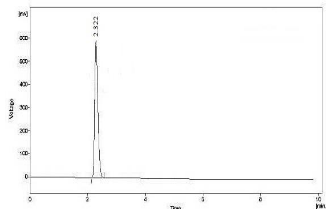
Fig. 3: Chromatogram of Olanzapine
