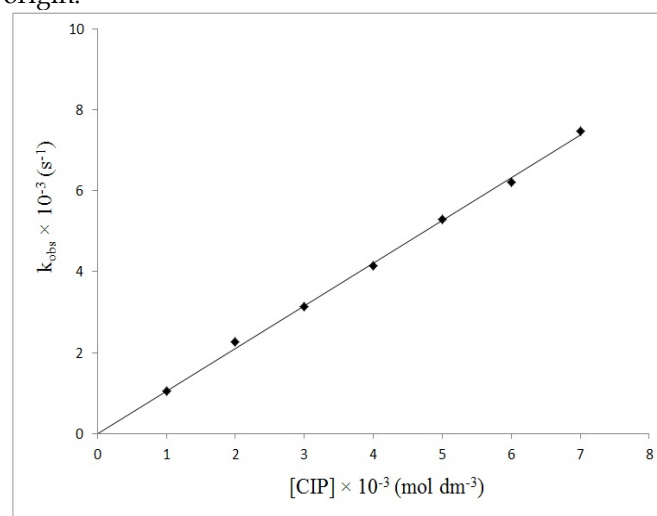
Fig. 4: Plot of [\text{CIP}] versus k_{\text{obs}} . [\text{KMnO}_4] = 2.5 \times 10^{-4} , [\text{H}^+] = 1.0 \times 10^{-2} , I = 5 \times 10^{-2}/\text{mol dm}^{-3} at 25°C.
