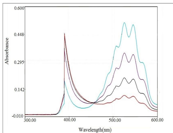
Fig. 5: Spectral changes during the oxidation of ciprofloxacin (CIP) by permanganate in acidic medium at 25^\circ\text{C} : [\text{MnO}_4^-] = 2.0 \times 10^{-4} , [\text{CIP}] = 2.0 \times 10^{-3} , [\text{H}^+] = 1.0 \times 10^{-2} and I = 0.05/\text{mol dm}^{-3} .
