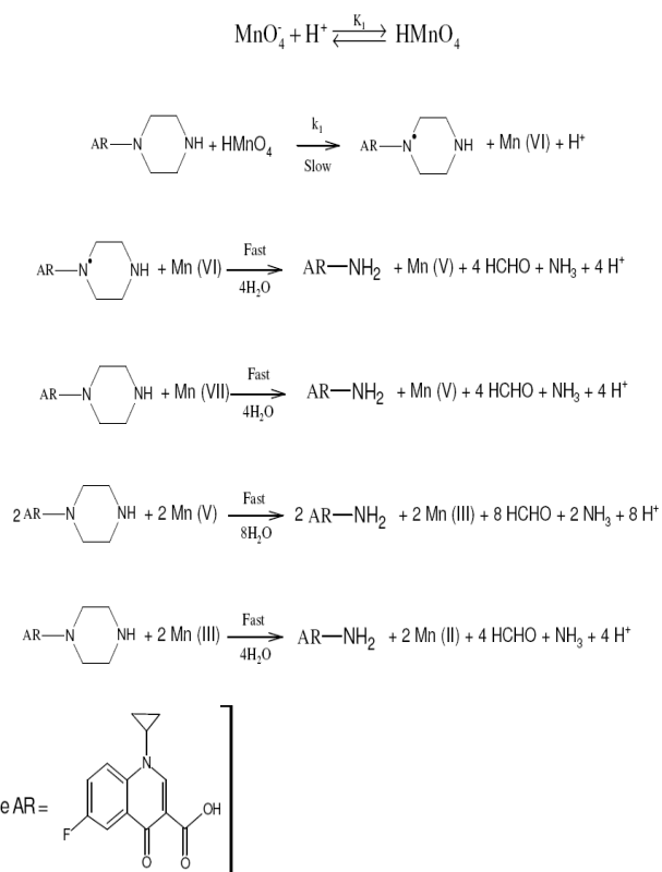
Scheme 1. Proposed mechanism for the oxidation of ciprofloxacin by acidic permanganate.
