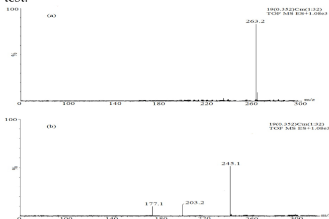
Fig. 1: LC-ESI-MS spectra of oxidation product of ciprofloxacin. (a) Molecular ion peak of m/z 263 (M-69). (b) Fragmentation of (M-69) product.
