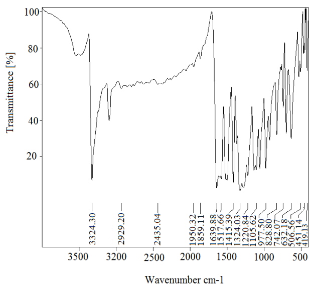
Fig. 2: FTIR spectra of the product of oxidation of ciprofloxacin by permanganate.
