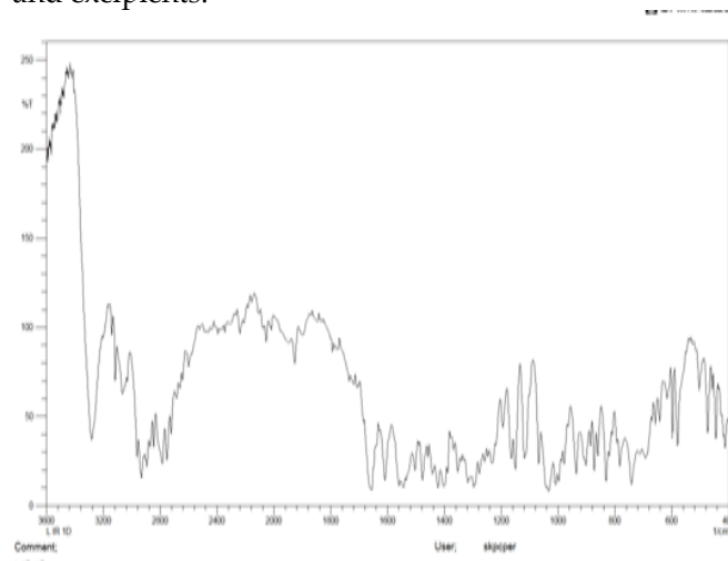
Fig. 2: FTIR Spectrum of Lafutidine
