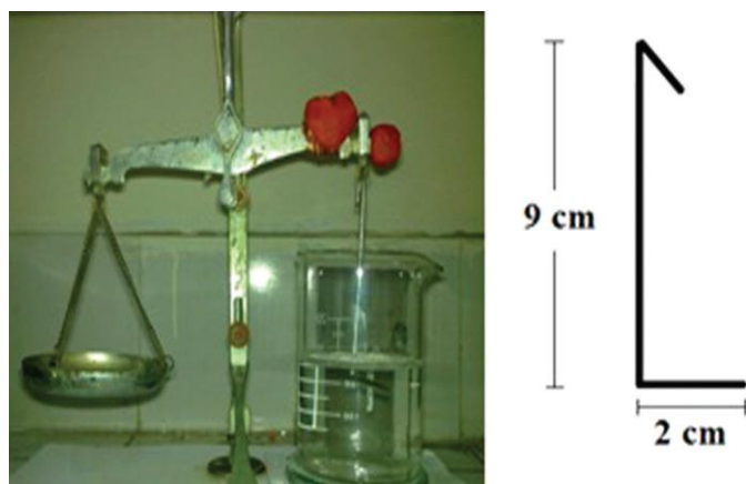
Fig. 1: (a) Modified balance method (b) Wire probe for raft strength measurement
