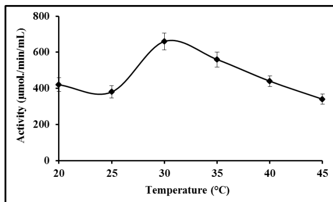
Fig. 5: Amylase activity for enzyme extract at various temperatures
