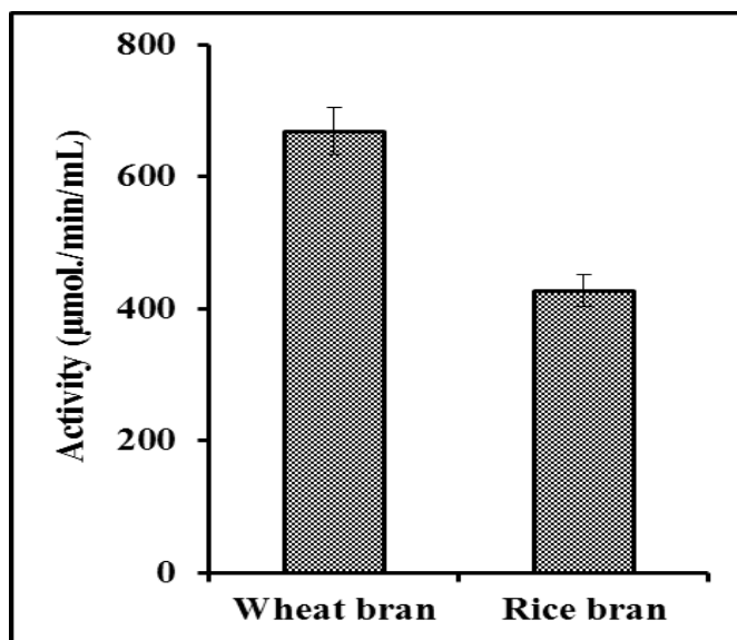
Fig. 1: Effect of substrate on \alpha -amylase production
