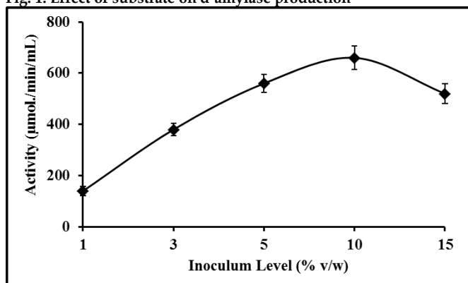
Fig. 2: Effect of different inoculum levels on \alpha -amylase production
