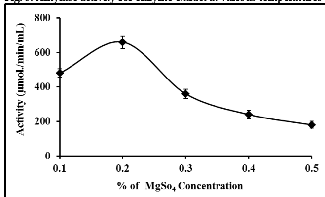
Fig. 6: Effect of different percentage of MgSO 4 on \alpha -amylase production
