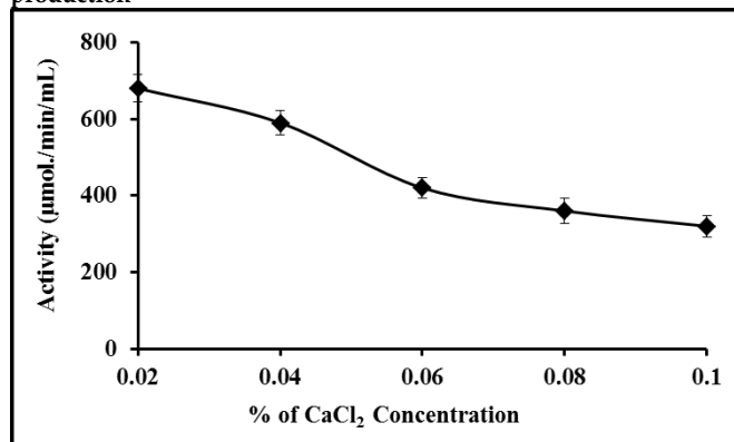
Fig. 7: Effect of different percentage of CaCl 2 on \alpha -amylase production
