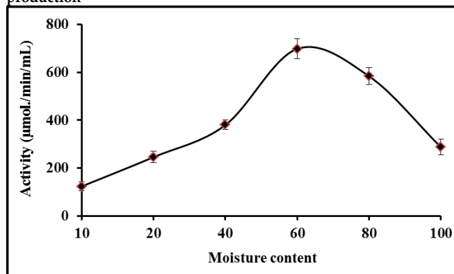
Fig. 8: Effect of different moisture content on \alpha -amylase production
