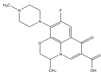
Fig. 1: Structure of Ofloxacin
