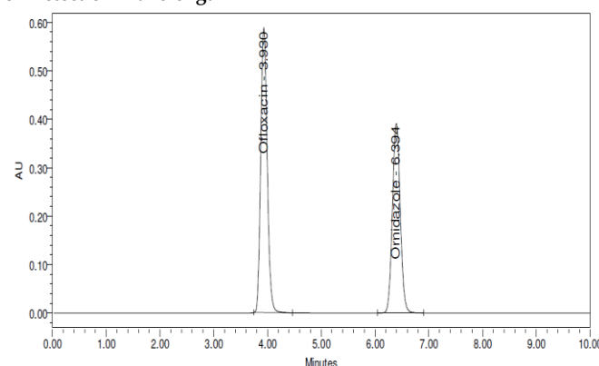
Fig. 4: Chromatogram of Standard OFL and ORN
