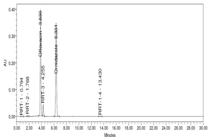
Fig. 6: Chromatogram of Tablet in Acidic condition
