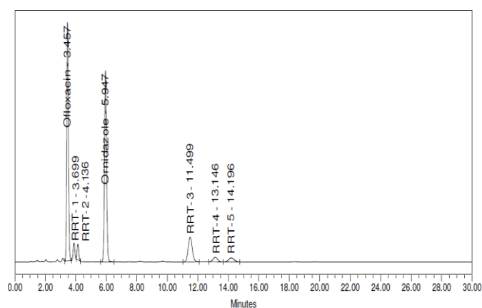
Fig. 9: Chromatogram of Tablet in Thermal condition
