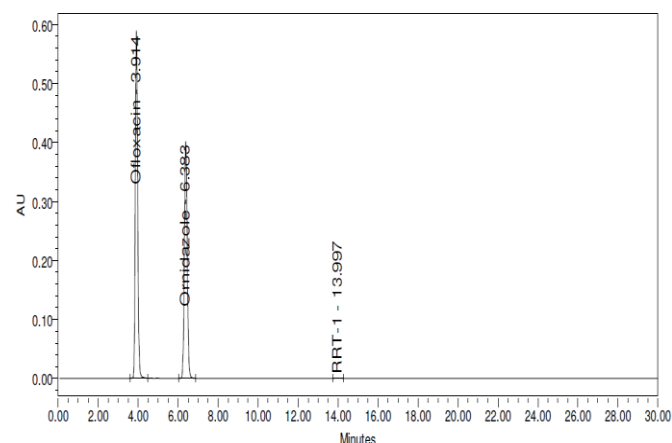
Fig. 10: Chromatogram of Tablet in photolytic condition
