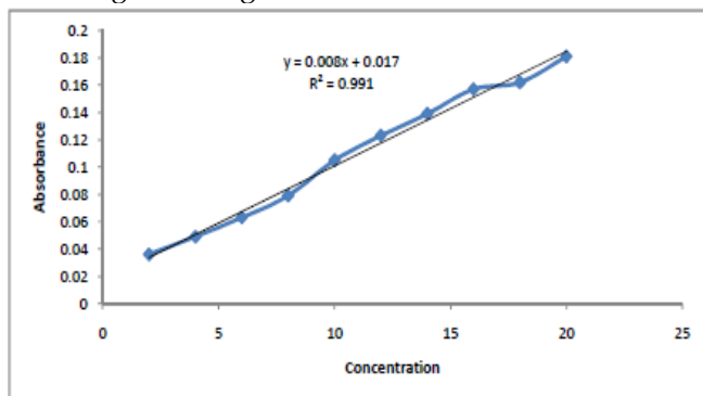
Fig. 2: Calibration curve of Azithromycin in PBS 6.8
