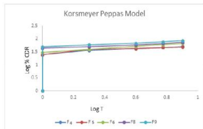
Fig. 15: Korsmeyer Peppas modeling of various formulations
