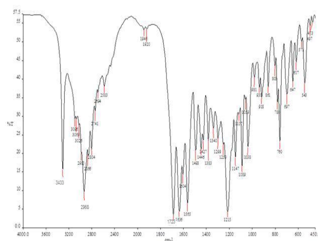
Fig. 3: FTIR spectrum of Azithromycin
