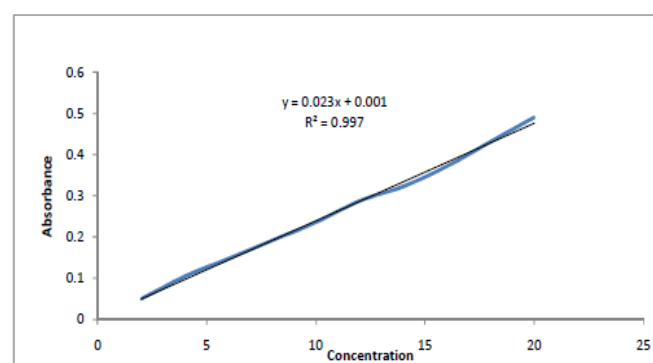
Fig. 1: Calibration curve of Azithromycin in 0.1 N HCl
