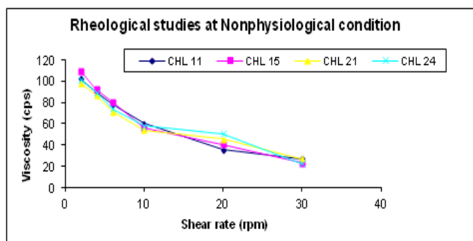
Fig. 4: Rheological studies of Formulations at Nonphysiological Condition (pH 5)
