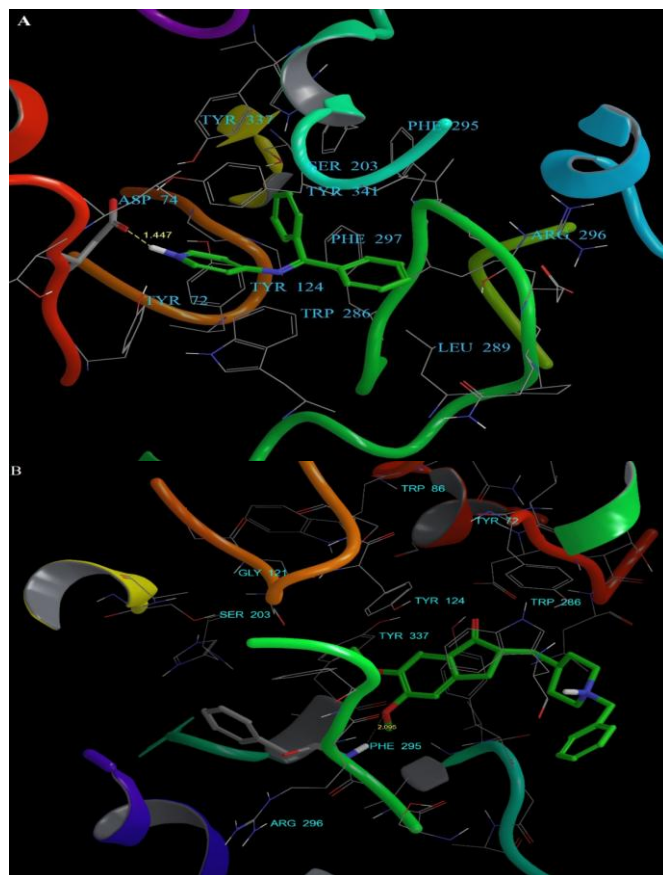
Fig. 1: The binding mode of [A] 4APg and [B] Donepezil in the AChE binding pocket. The hydrogen bonds are displayed as dashed yellow
