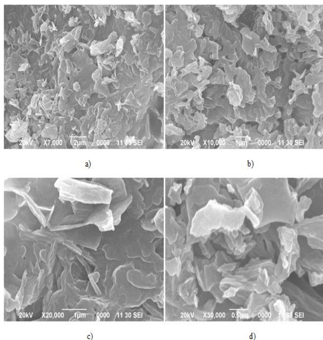
Fig. 4: SEM Images of ZnO NP's synthesized from Calotropis procera
