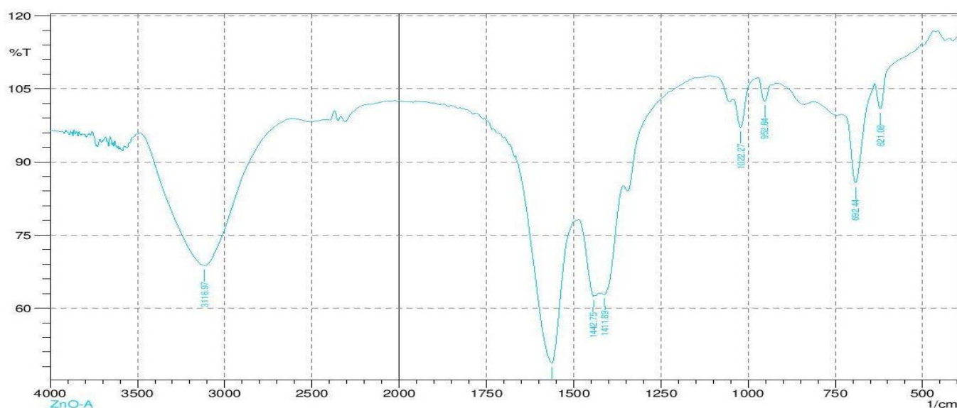
Fig. 3: FTIR Spectrum of ZnO NP's synthesized from Calotropis procera
