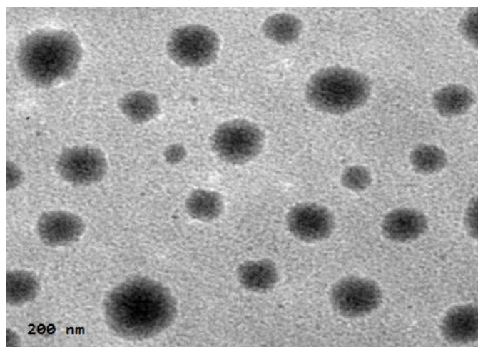
Fig. 5: Transmission electron microscopic image of optimized Rifampicin nanoemulsion (A3)
