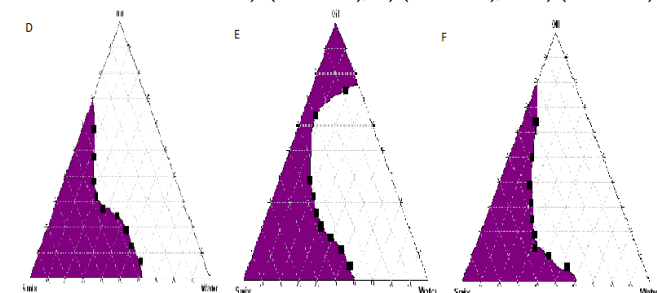
Fig. 2: Pseudo Ternary phase diagram of capryol 90, tween 80, transcutool P and water D). (Smix 1:1), E) (Smix 1:2), & F) (Smix 1:3)
