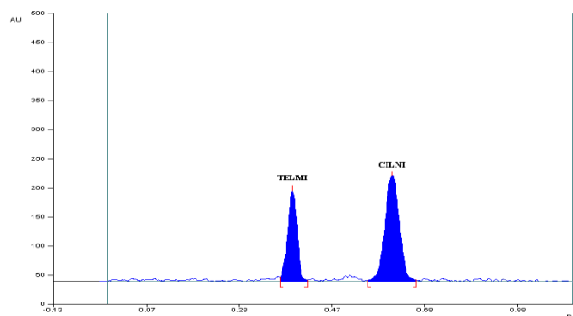
Fig. 1: Representative densitogram of mixed standard solution of TELMI (600 ng band -1 , R_f = 0.38 \pm 0.03 ) and CILNI (300 ng band -1 , R_f = 0.62 \pm 0.05 )
