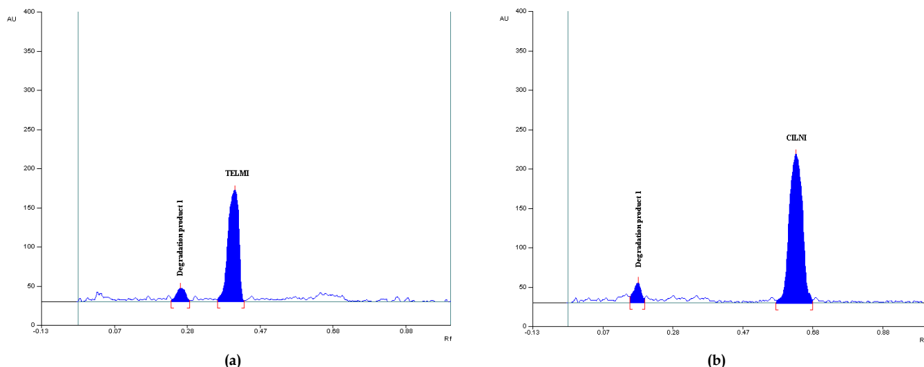
Fig. 6: Densitogram obtained from sample (a) TELMI (b) CILNI subjected to dry heat
