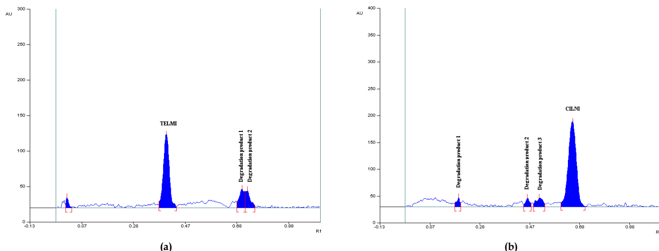
Fig. 5: Representative densitogram after oxidative degradation (a) TELMI with degradation products at Rf 0.70, 0.74 (b) CILNI with degradation products at Rf 0.20, 0.45, 0.50
