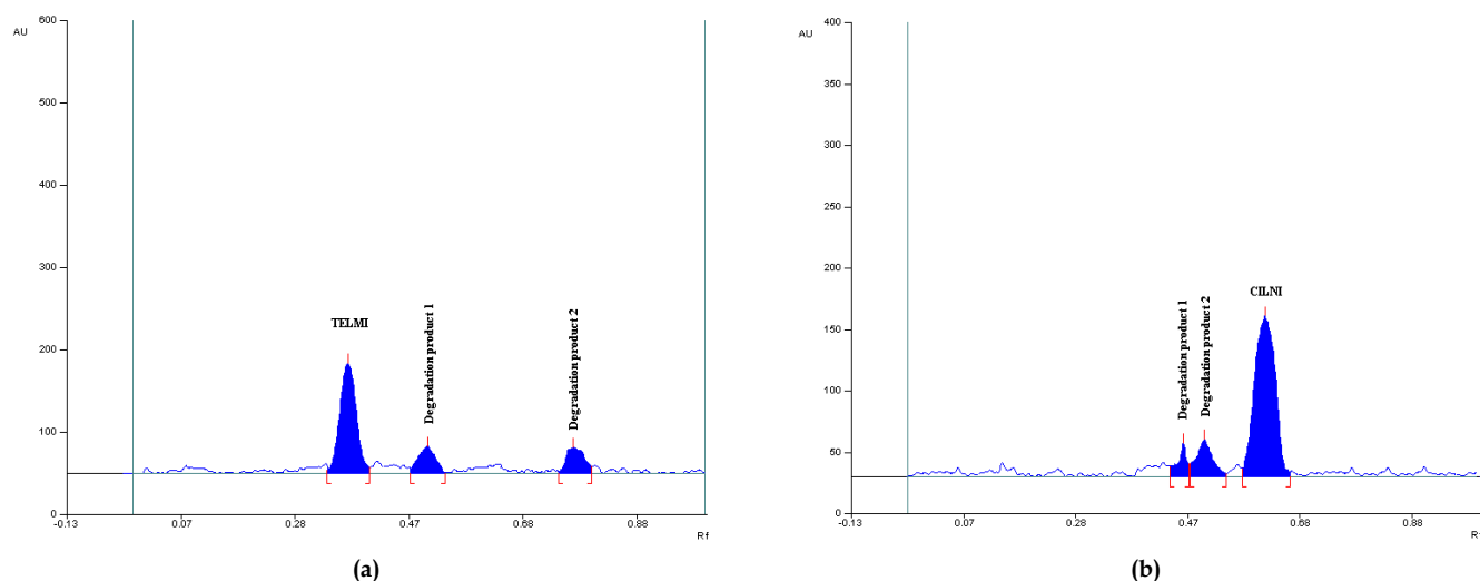
Fig. 4: Representative densitogram obtained after neutral degradation with (a) TELMI with degradation products at Rf 0.50, 0.77 (b) CILNI with degradation products at Rf 0.46, 0.52
