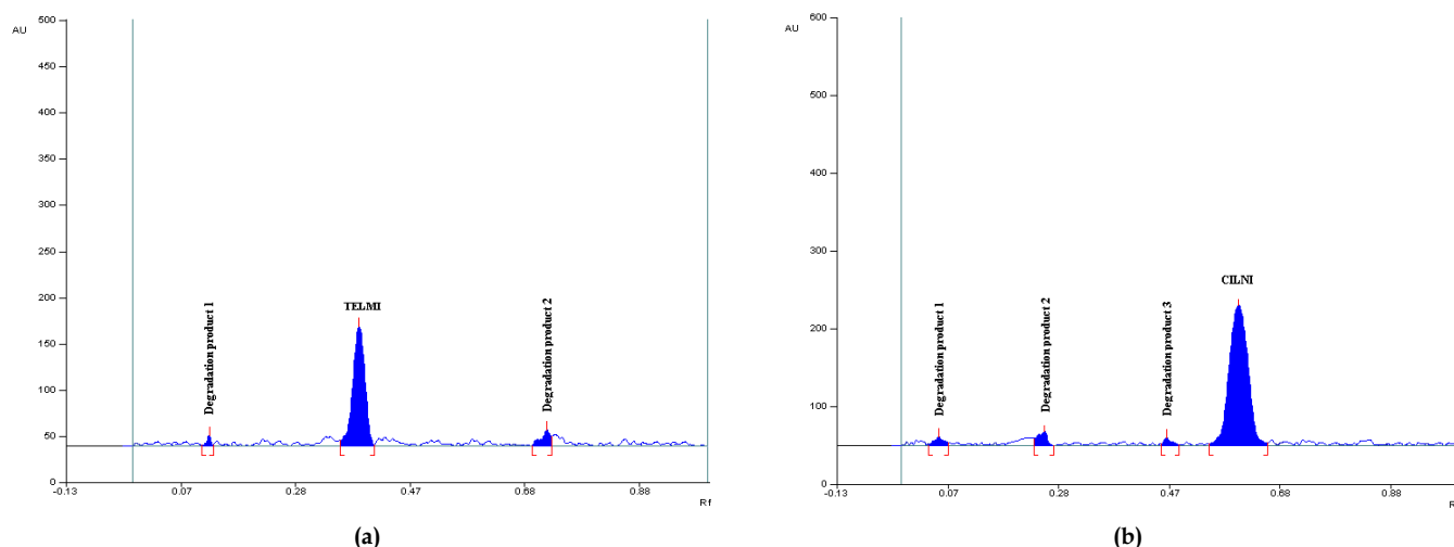
Fig. 2: Representative densitogram after acid treatment (a) TELMI with degradation products at Rf 0.13, 0.71 and (b) CILNI with degradation products at Rf 0.06, 0.26 and 0.47
