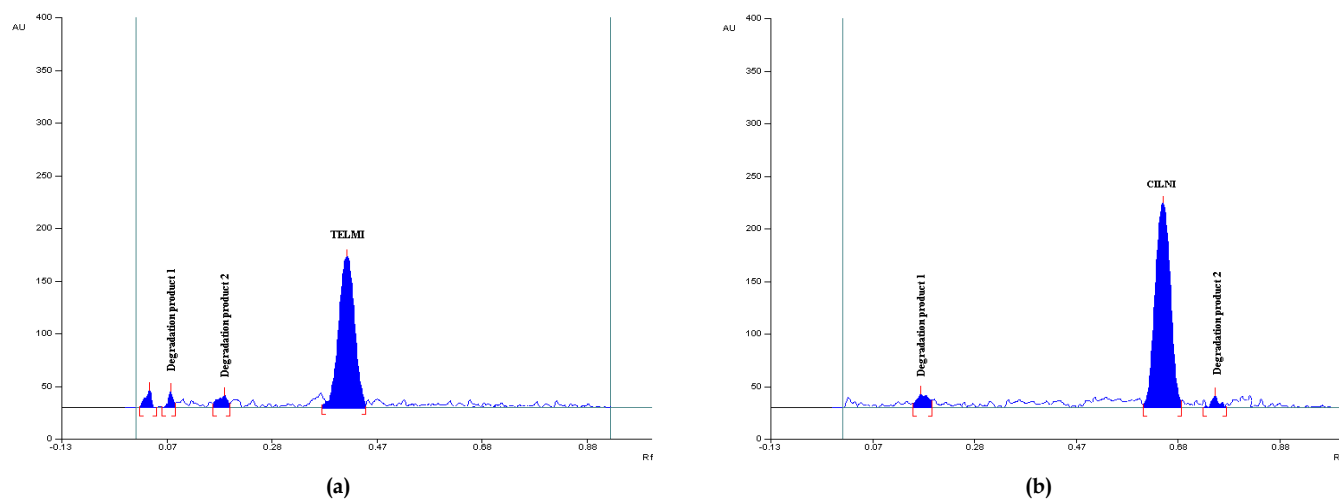
Fig. 3: Representative densitogram after alkali treatment (a) TELMI with degradation products at Rf 0.08, 0.18 and (b) CILNI with degradation products at Rf 0.18 and 0.74
