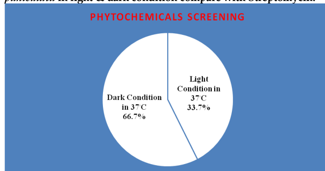
Fig. 4: Phytochemical screening of Isopropanol extract of A. paniculata
