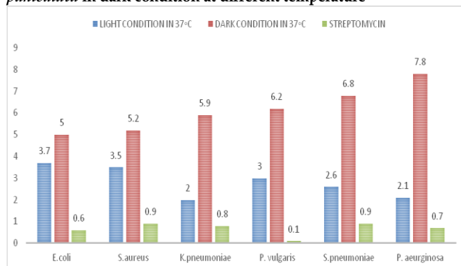
Fig. 3: Zones of inhibition (mm) by Isopropanol extract of A. paniculata in light & dark condition compare with Streptomycin.
