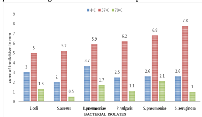
Fig. 2: Zones of inhibition (mm) by Isopropanol extract of A. paniculata in dark condition at different temperature
