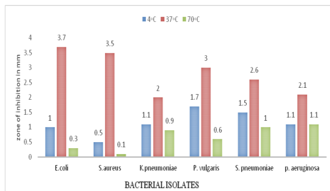
Fig. 1: Zones of inhibition (mm) by Isopropanol extract of A. paniculata in light condition at different temperature
