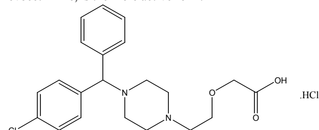
Fig. 3: Structure of Cetirizine hydrochloride
