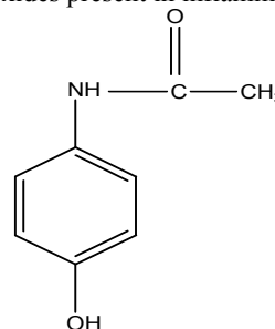
Fig. 1: Structure of Paracetamol
