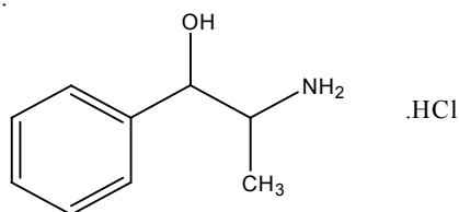
Fig. 2: Structure of Phenylpropanolamine hydrochloride
