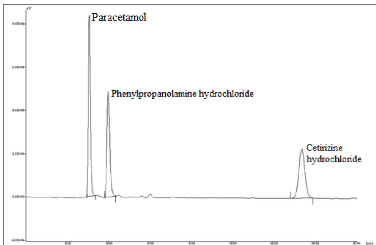
Fig. 4: Chromatogram of Paracetamol R_t (3.108), Phenylpropanolamine hydrochloride R_t (4.008) and Cetirizine hydrochloride R_t (13.392)
