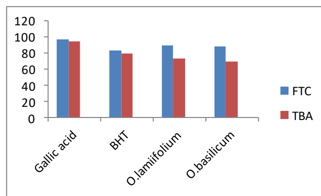
Fig. 1: Antioxidant properties of plant extract compared to the standards (Gallic acid and BHT) as determined with the FTC (500 nm) and TBA (552 nm) methods on the 7th day. TBA: Thiobarbituric acid. FTC: Ferric thiocyanate. BHT: Butylated hydroxyl toluene.
