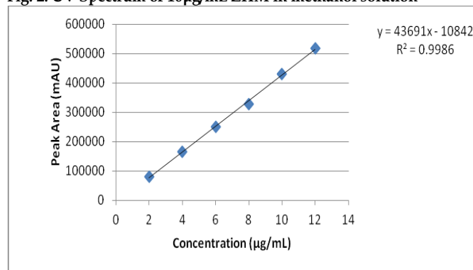
Fig. 3: Calibration Curve Indicating Linearity for ZHM
