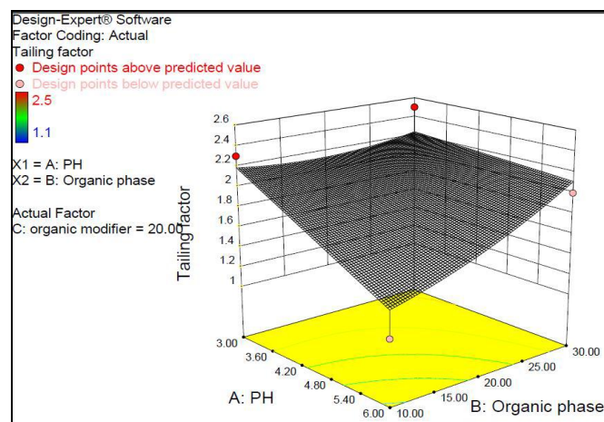
Fig. 5: 3D Response-Surface Graphs for Tailing Factor
