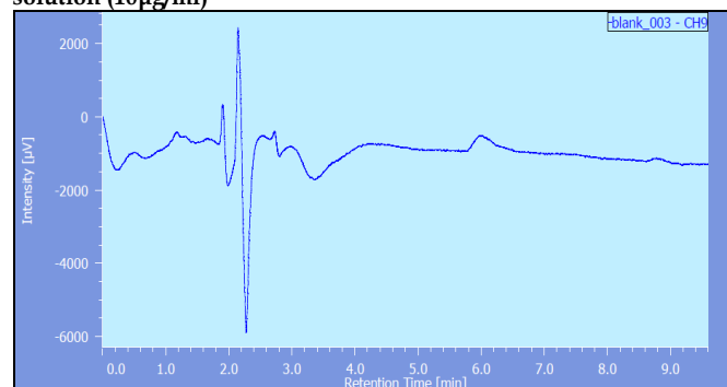
Fig. 7: Chromatogram of Blank run
