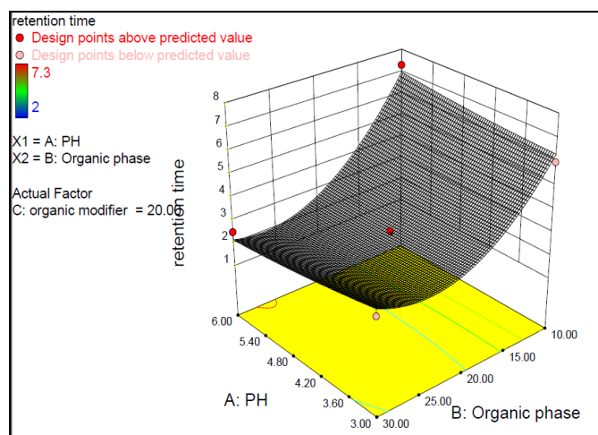
Fig. 3: 3D Response-Surface Graphs for Retention Time
