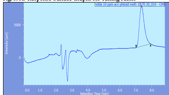
Fig. 6: Representative Chromatogram for Vildagliptin standard solution (10µg/ml)
