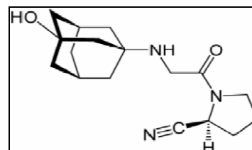
Fig. 1: Chemical structure of Vildagliptin
