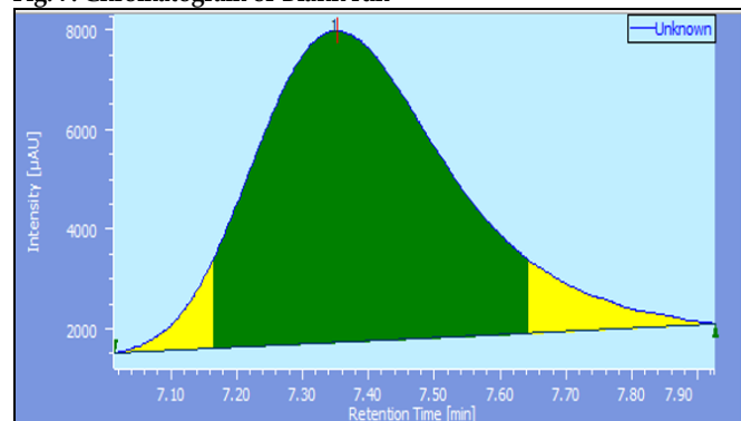
Fig. 8: Peak Purity for Vildagliptin solution (10µg/ml)
