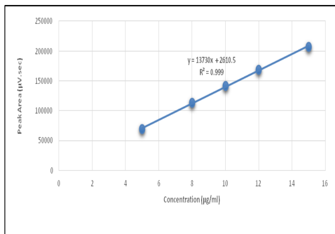
Fig. 9: Calibration Curve for Vildagliptin
