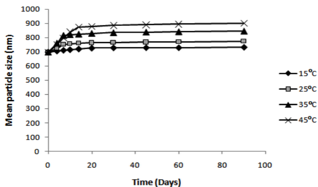
Fig. 5: Relative size of PVP formulations at different temperature
