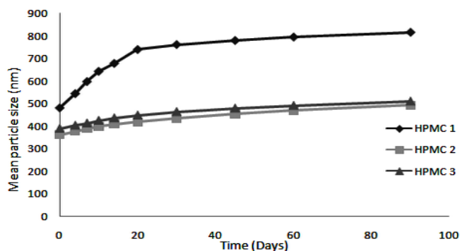
Fig. 2: Mean particle size of HPMC formulations at 45°C as a function of time
