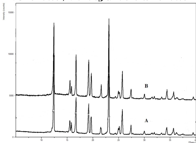
Fig. 9: Powder X-ray diffraction pattern of esomeprazole. A. Raw drug, B. Pluronic F68-2 formulation
