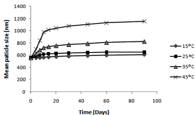
Fig. 3: Mean particle size of HPC 1 formulation as a function of temperature and time
