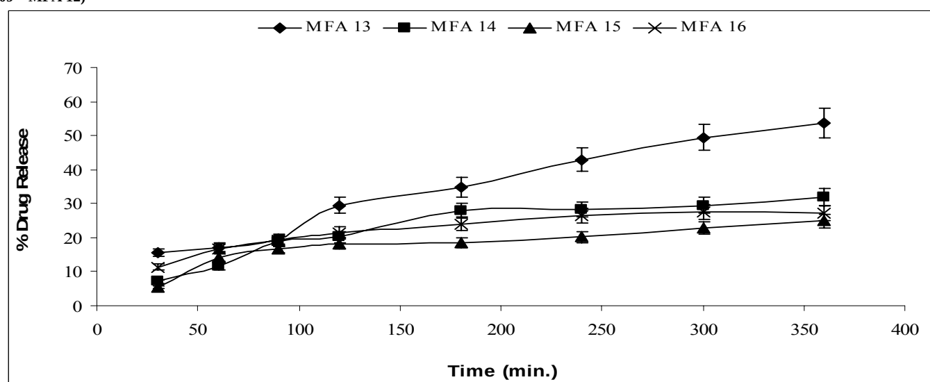
Fig. 7: Dissolution profile of pure Mefenamic acid (MFA-16) and its formulations prepared by melt mixing (MFA-13 – MFA-15)
