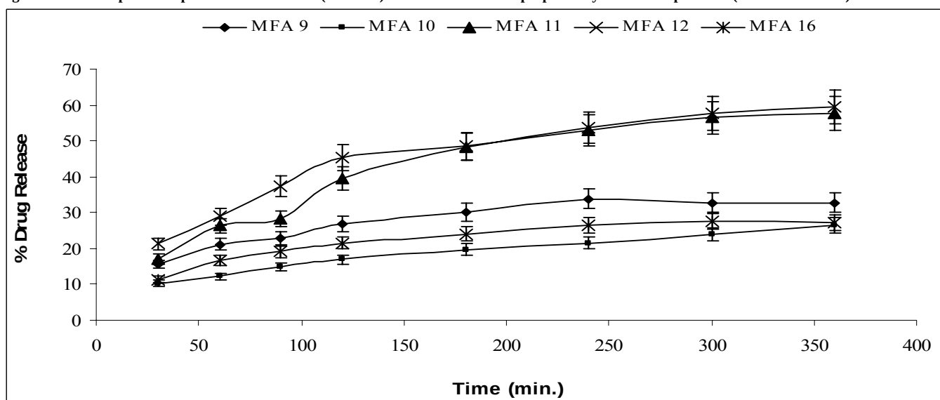
Fig. 6: Dissolution profile of pure Mefenamic acid (MFA-16) and its formulations prepared by evaporative precipitation into aqueous solution (MFA-9 – MFA-12)
