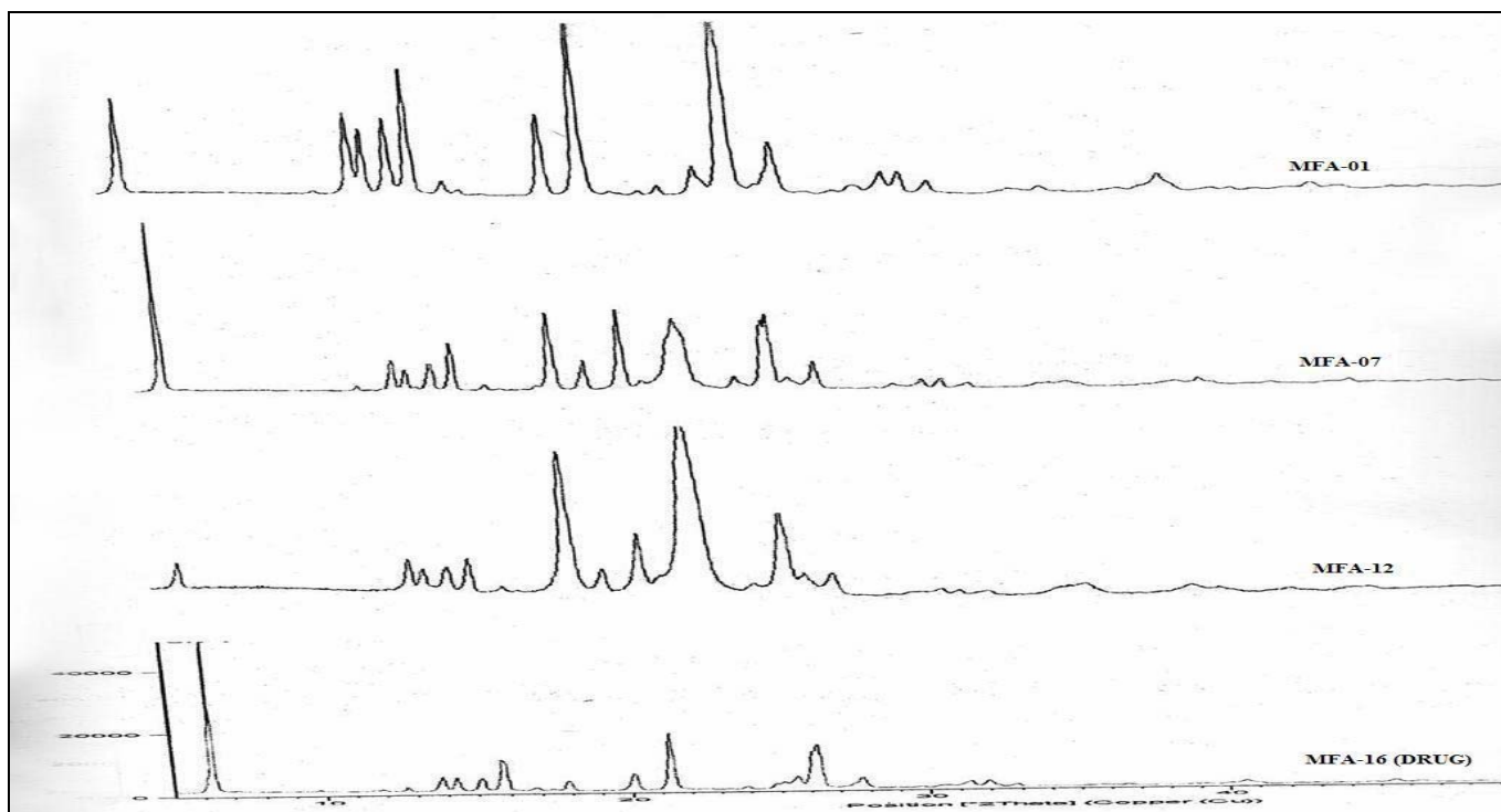
Fig. 2: Powder X-Ray diffraction spectra of pure Mefenamic acid, MFA-01, MFA-07 and MFA-12
