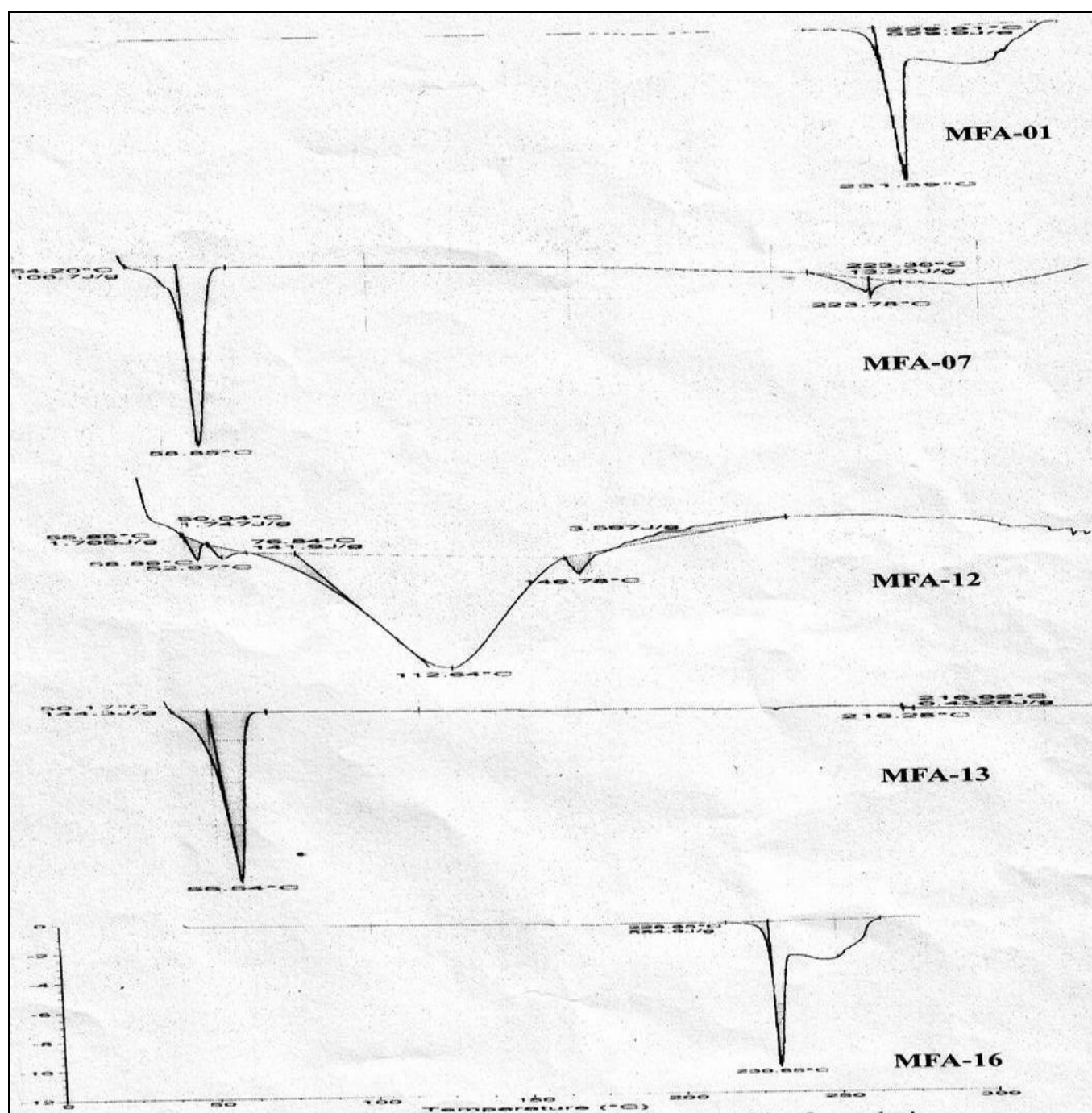
Fig. 1: DSC thermogram of pure Mefenamic acid and its formulations
